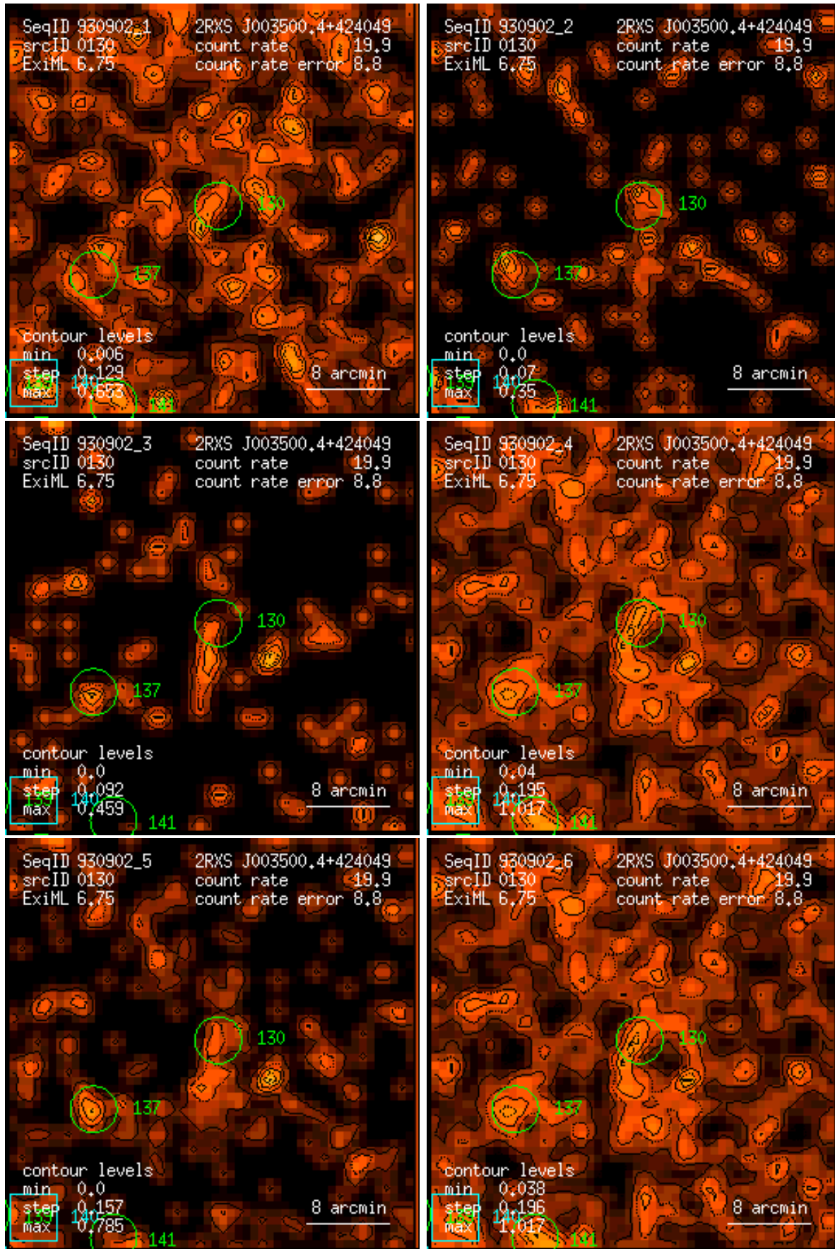
Figure 130: RASS 930902: detection 0130: band rate images, Gaussian filter: (1) PSPC channels 11 – 41, (2) 52 – 90, (3) 91 – 201, (4) 11 – 235, (5) 52 – 201, (6) 11 – 201. Broad band rates in counts/ks. Band rate contour levels in counts/ks/arcmin 2 .
