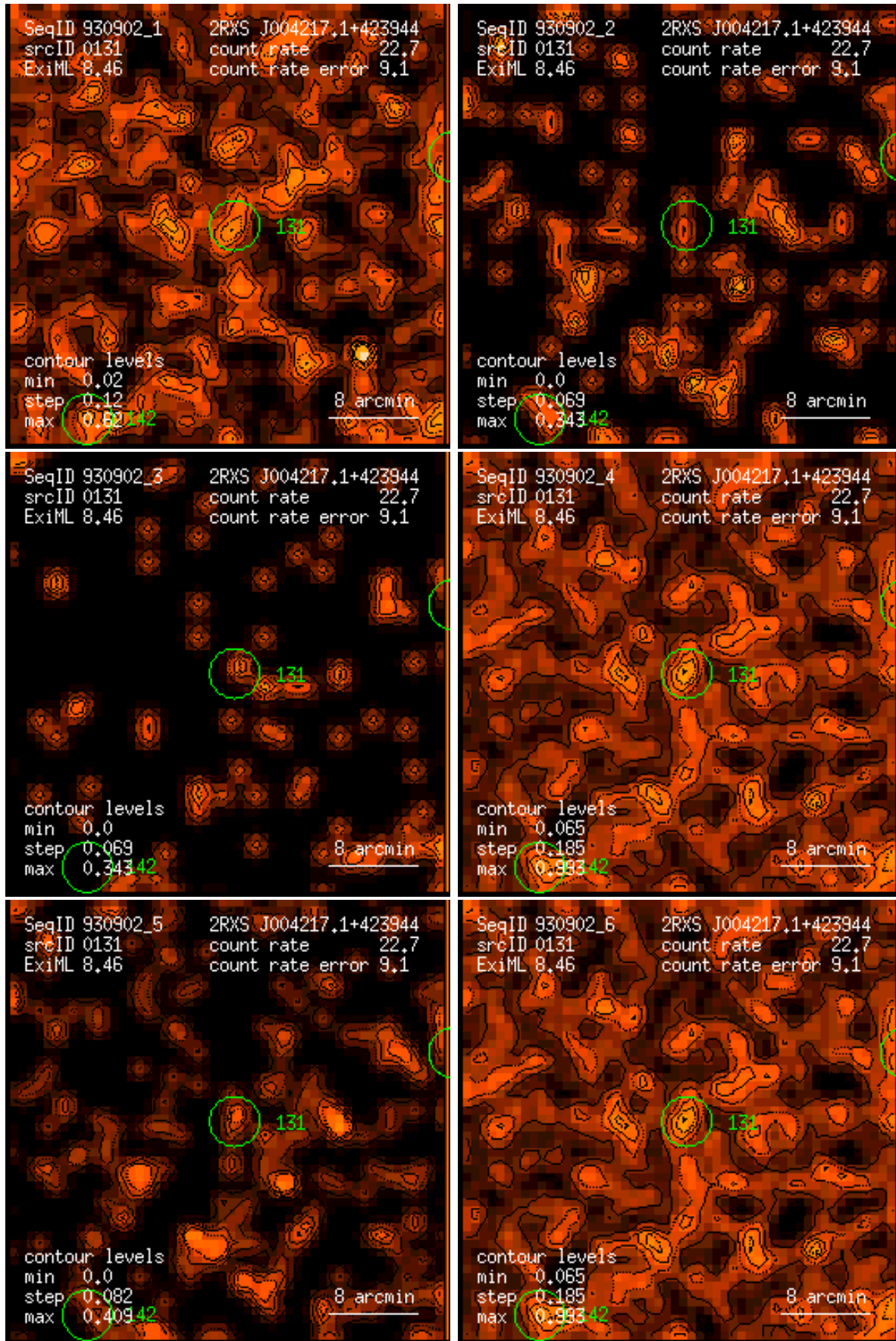
Figure 131: RASS 930902: detection 0131: band rate images, Gaussian filter: (1) PSPC channels 11 – 41, (2) 52 – 90, (3) 91 – 201, (4) 11 – 235, (5) 52 – 201, (6) 11 – 201. Broad band rates in counts/ks. Band rate contour levels in counts/ks/arcmin 2 .
