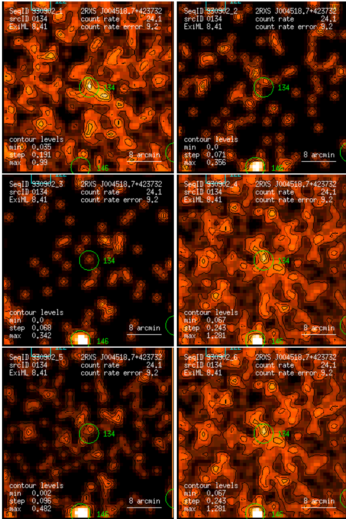
Figure 134: RASS 930902: detection 0134: band rate images, Gaussian filter: (1) PSPC channels 11 – 41, (2) 52 – 90, (3) 91 – 201, (4) 11 – 235, (5) 52 – 201, (6) 11 – 201. Broad band rates in counts/ks. Band rate contour levels in counts/ks/arcmin 2 .
