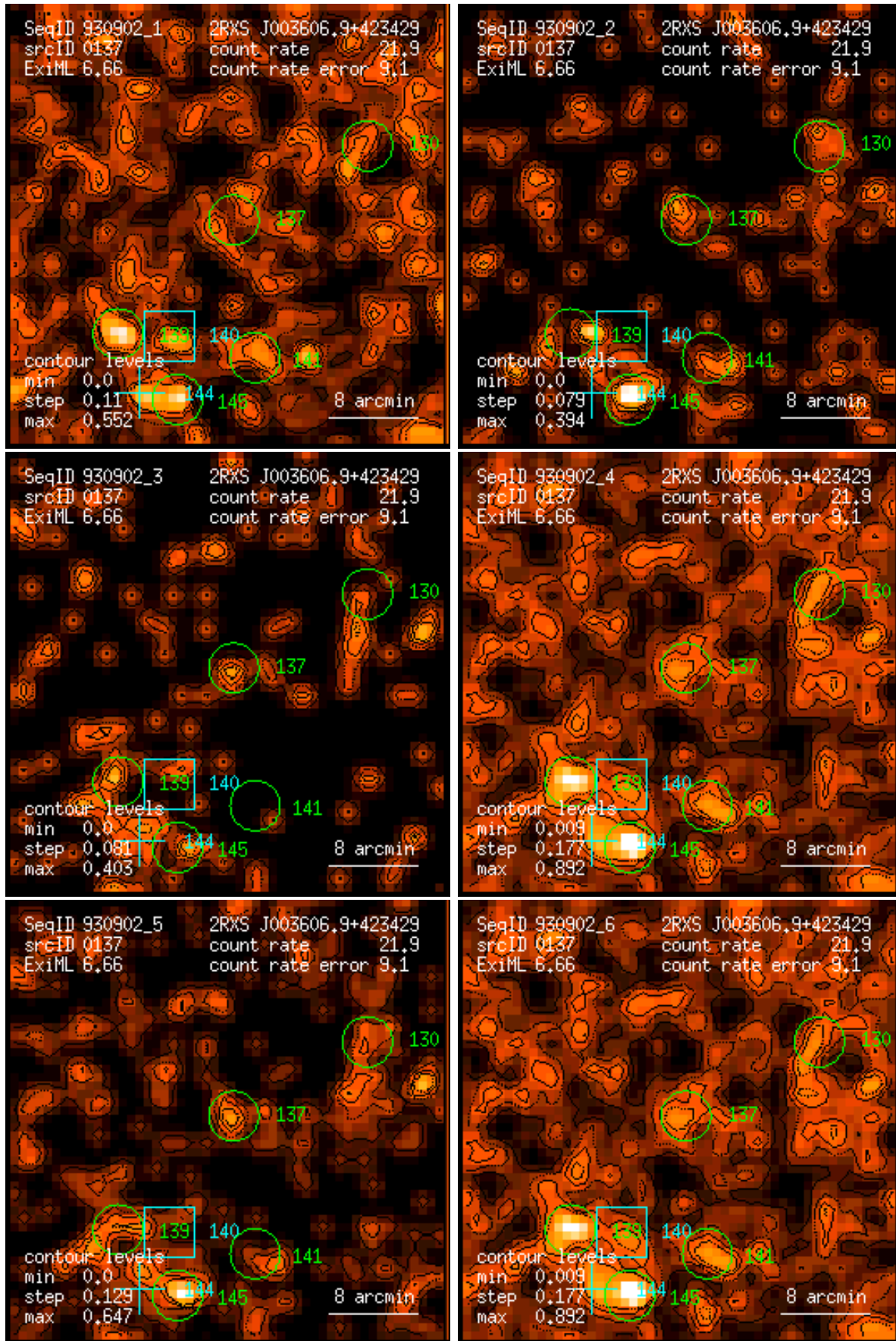
Figure 137: RASS 930902: detection 0137: band rate images, Gaussian filter: (1) PSPC channels 11 – 41, (2) 52 – 90, (3) 91 – 201, (4) 11 – 235, (5) 52 – 201, (6) 11 – 201. Broad band rates in counts/ks. Band rate contour levels in counts/ks/arcmin 2 .
