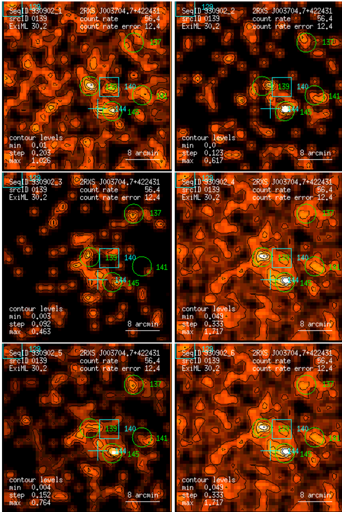
Figure 139: RASS 930902: detection 0139: band rate images, Gaussian filter: (1) PSPC channels 11 – 41, (2) 52 – 90, (3) 91 – 201, (4) 11 – 235, (5) 52 – 201, (6) 11 – 201. Broad band rates in counts/ks. Band rate contour levels in counts/ks/arcmin 2 .
