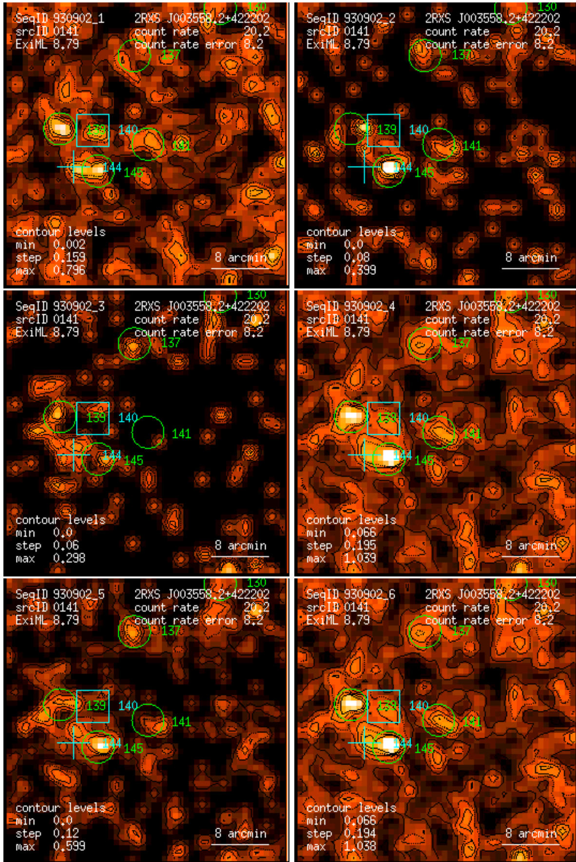
Figure 141: RASS 930902: detection 0141: band rate images, Gaussian filter: (1) PSPC channels 11 – 41, (2) 52 – 90, (3) 91 – 201, (4) 11 – 235, (5) 52 – 201, (6) 11 – 201. Broad band rates in counts/ks. Band rate contour levels in counts/ks/arcmin 2 .
