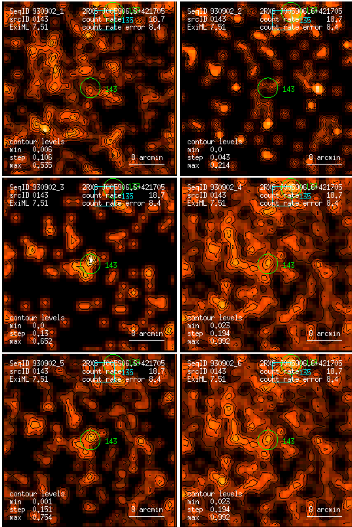
Figure 143: RASS 930902: detection 0143: band rate images, Gaussian filter: (1) PSPC channels 11 – 41, (2) 52 – 90, (3) 91 – 201, (4) 11 – 235, (5) 52 – 201, (6) 11 – 201. Broad band rates in counts/ks. Band rate contour levels in counts/ks/arcmin 2 .
