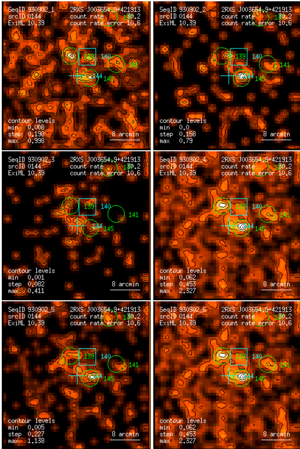
Figure 144: RASS 930902: detection 0144: band rate images, Gaussian filter: (1) PSPC channels 11 – 41, (2) 52 – 90, (3) 91 – 201, (4) 11 – 235, (5) 52 – 201, (6) 11 – 201. Broad band rates in counts/ks. Band rate contour levels in counts/ks/arcmin 2 .
