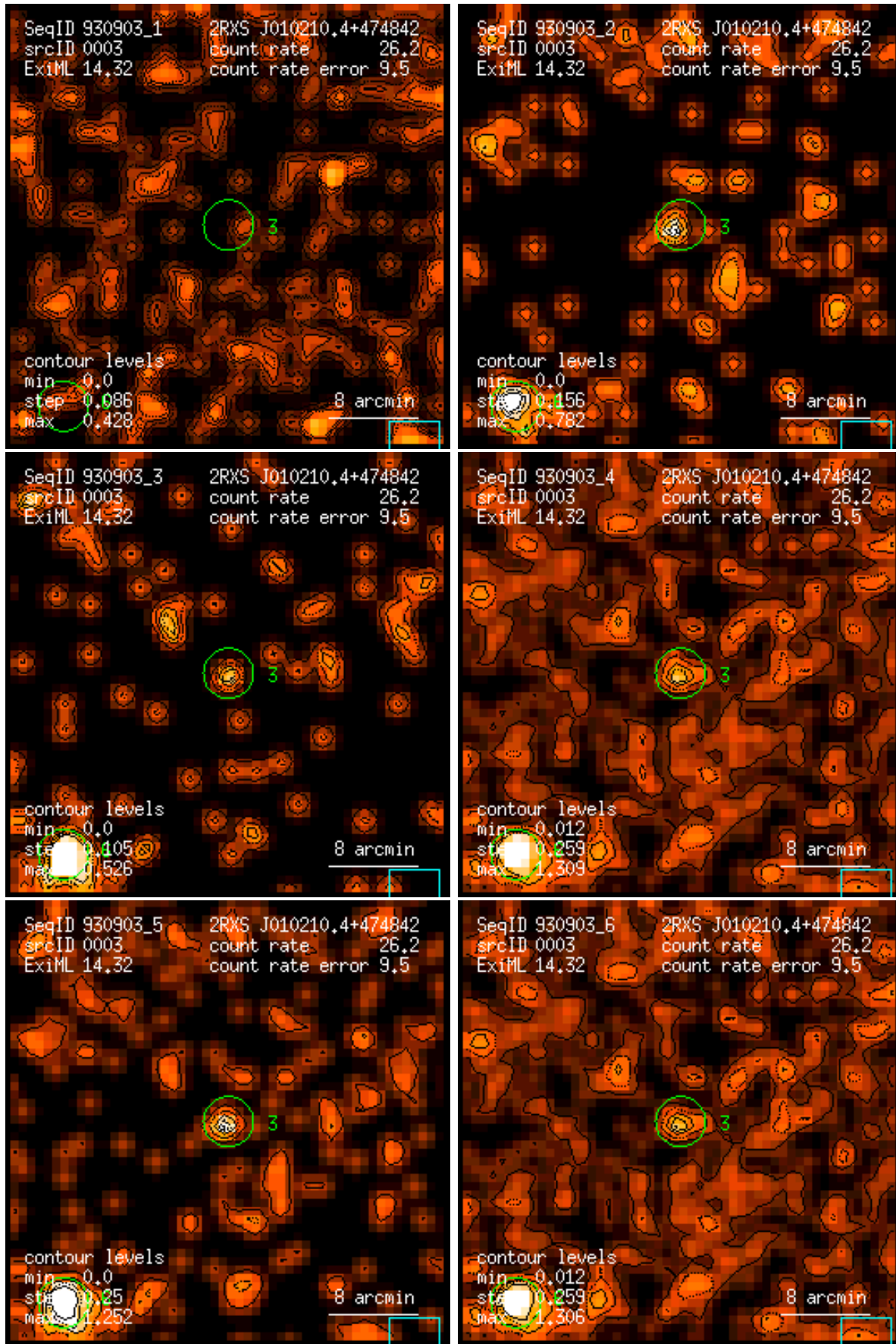
Figure 3: RASS 930903: detection 0003: band rate images, Gaussian filter: (1) PSPC channels 11 – 41, (2) 52 – 90, (3) 91 – 201, (4) 11 – 235, (5) 52 – 201, (6) 11 – 201. Broad band rates in counts/ks. Band rate contour levels in counts/ks/arcmin 2 .
