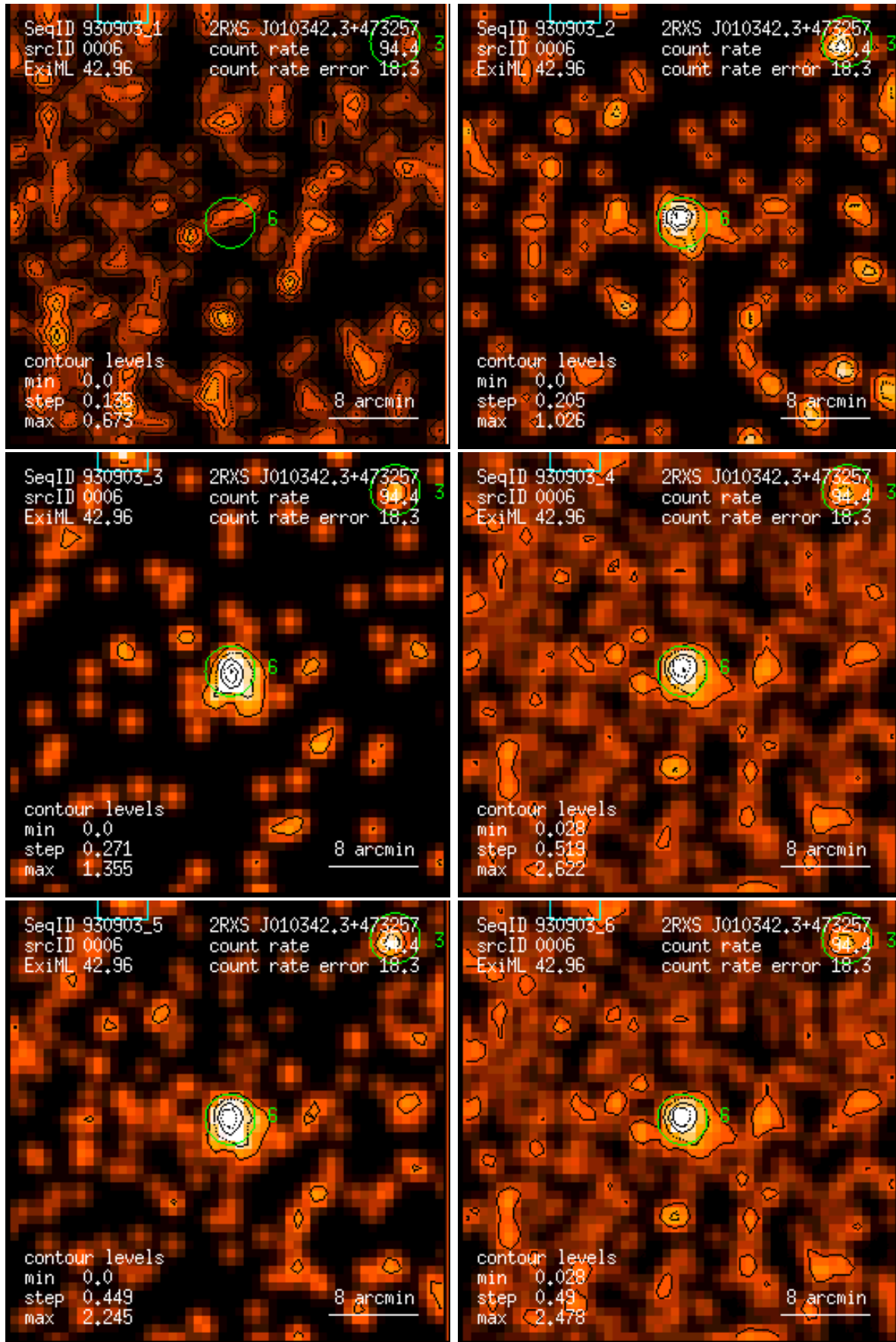
Figure 6: RASS 930903: detection 0006: band rate images, Gaussian filter: (1) PSPC channels 11 – 41, (2) 52 – 90, (3) 91 – 201, (4) 11 – 235, (5) 52 – 201, (6) 11 – 201. Broad band rates in counts/ks. Band rate contour levels in counts/ks/arcmin 2 .
