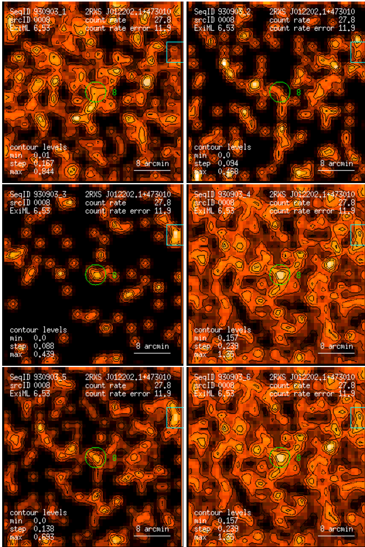
Figure 8: RASS 930903: detection 0008: band rate images, Gaussian filter: (1) PSPC channels 11 – 41, (2) 52 – 90, (3) 91 – 201, (4) 11 – 235, (5) 52 – 201, (6) 11 – 201. Broad band rates in counts/ks. Band rate contour levels in counts/ks/arcmin 2 .
