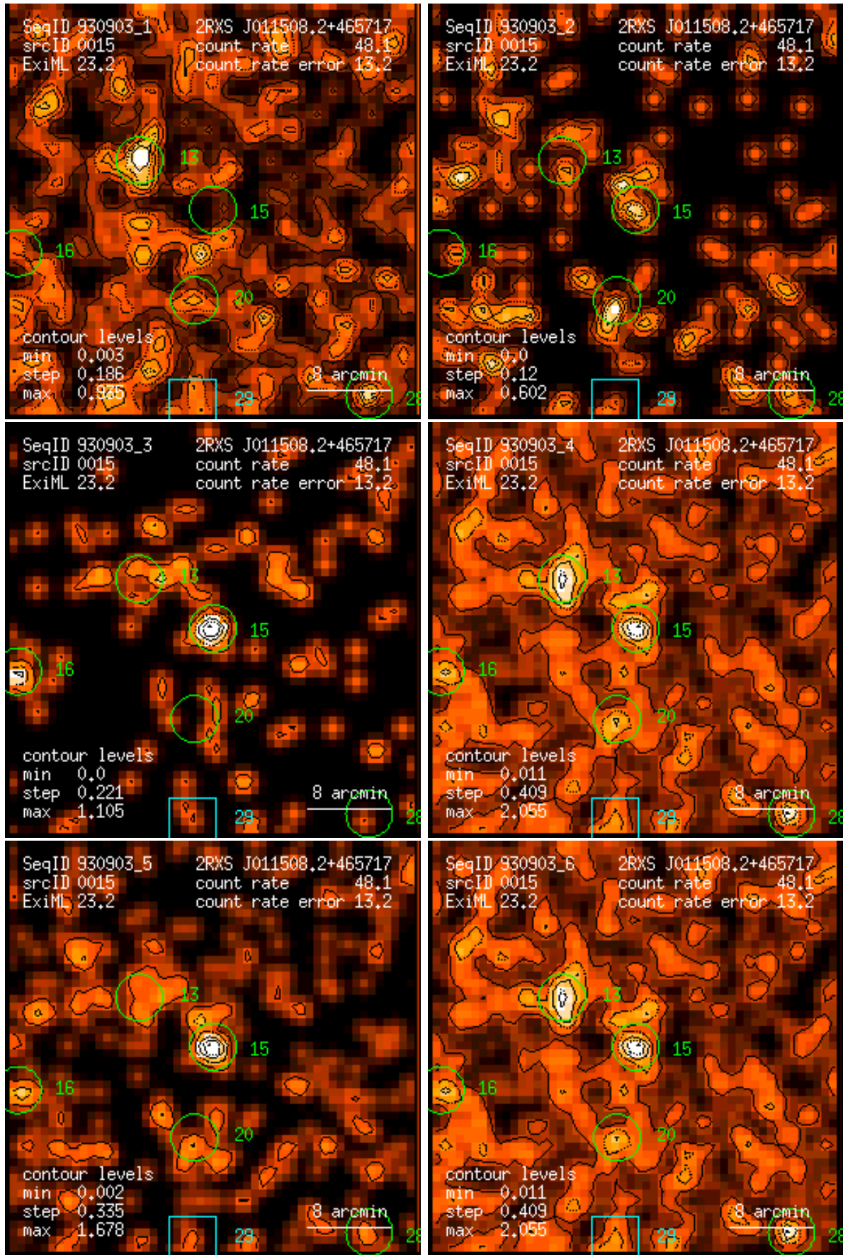
Figure 15: RASS 930903: detection 0015: band rate images, Gaussian filter: (1) PSPC channels 11 – 41, (2) 52 – 90, (3) 91 – 201, (4) 11 – 235, (5) 52 – 201, (6) 11 – 201. Broad band rates in counts/ks. Band rate contour levels in counts/ks/arcmin 2 .
