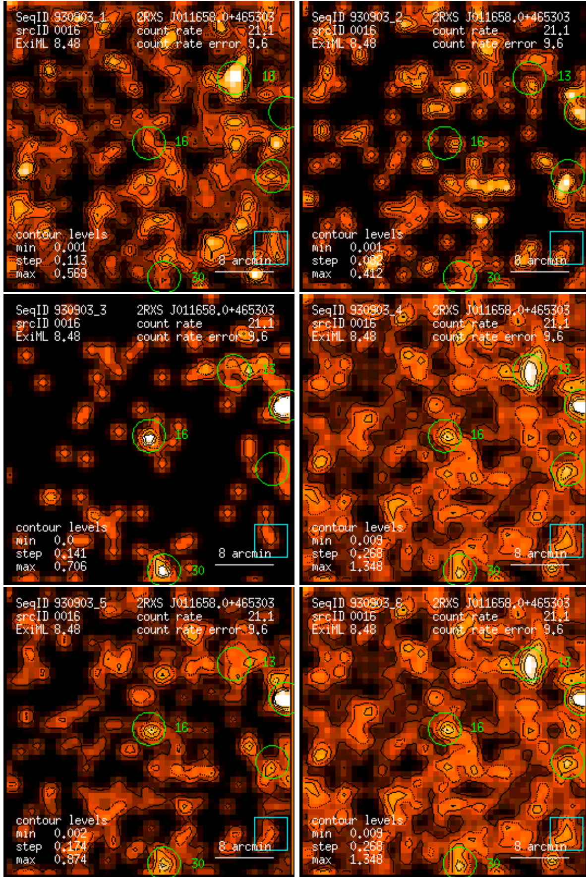
Figure 16: RASS 930903: detection 0016: band rate images, Gaussian filter: (1) PSPC channels 11 – 41, (2) 52 – 90, (3) 91 – 201, (4) 11 – 235, (5) 52 – 201, (6) 11 – 201. Broad band rates in counts/ks. Band rate contour levels in counts/ks/arcmin 2 .
