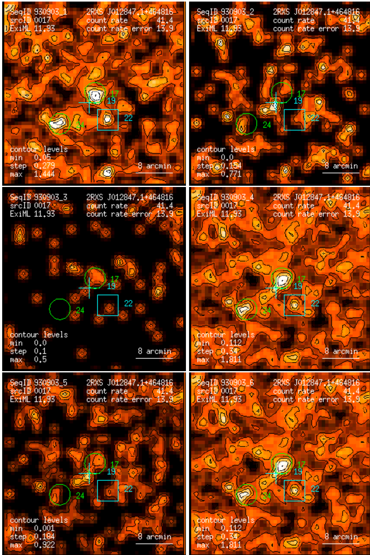
Figure 17: RASS 930903: detection 0017: band rate images, Gaussian filter: (1) PSPC channels 11 – 41, (2) 52 – 90, (3) 91 – 201, (4) 11 – 235, (5) 52 – 201, (6) 11 – 201. Broad band rates in counts/ks. Band rate contour levels in counts/ks/arcmin 2 .
