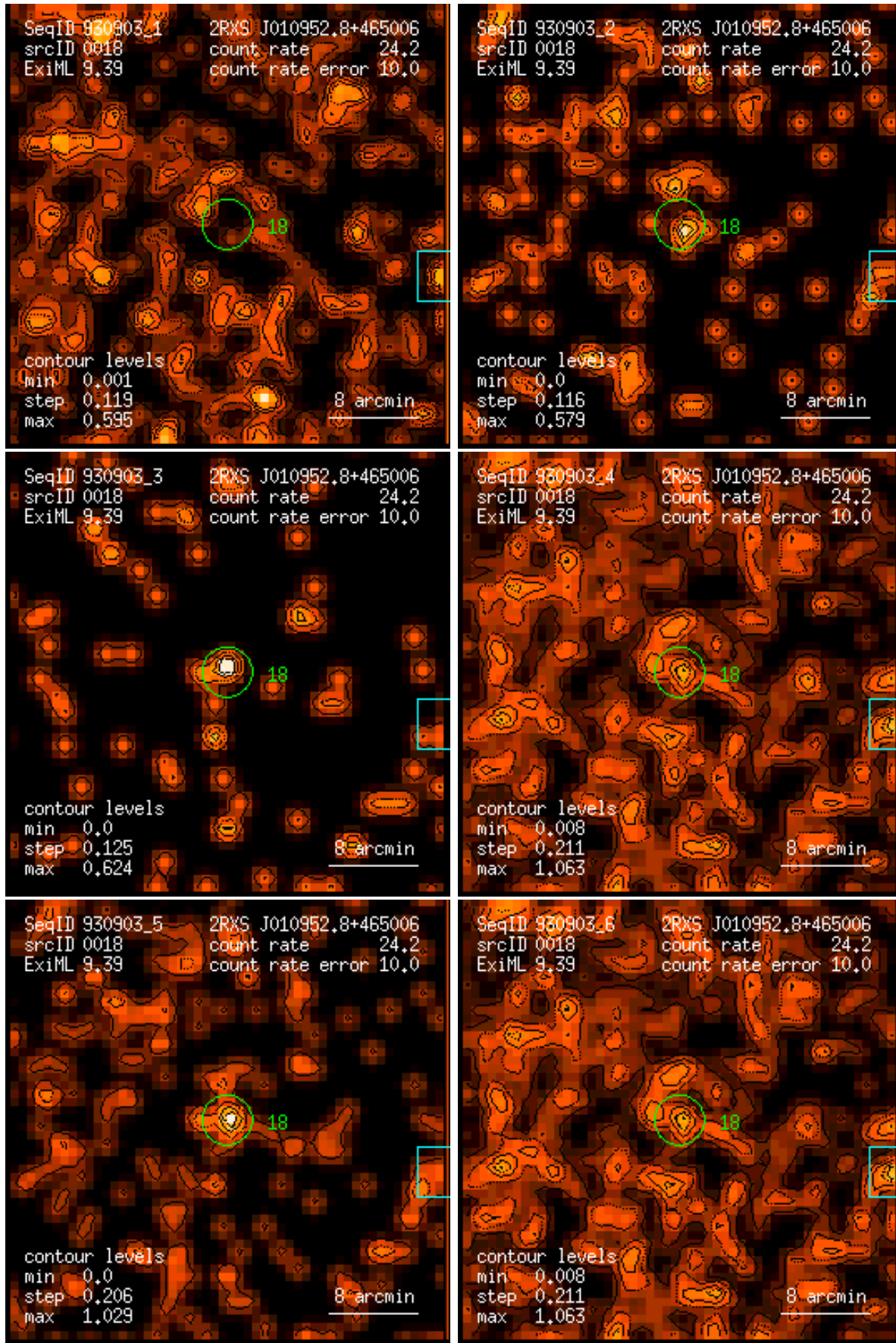
Figure 18: RASS 930903: detection 0018: band rate images, Gaussian filter: (1) PSPC channels 11 – 41, (2) 52 – 90, (3) 91 – 201, (4) 11 – 235, (5) 52 – 201, (6) 11 – 201. Broad band rates in counts/ks. Band rate contour levels in counts/ks/arcmin 2 .
