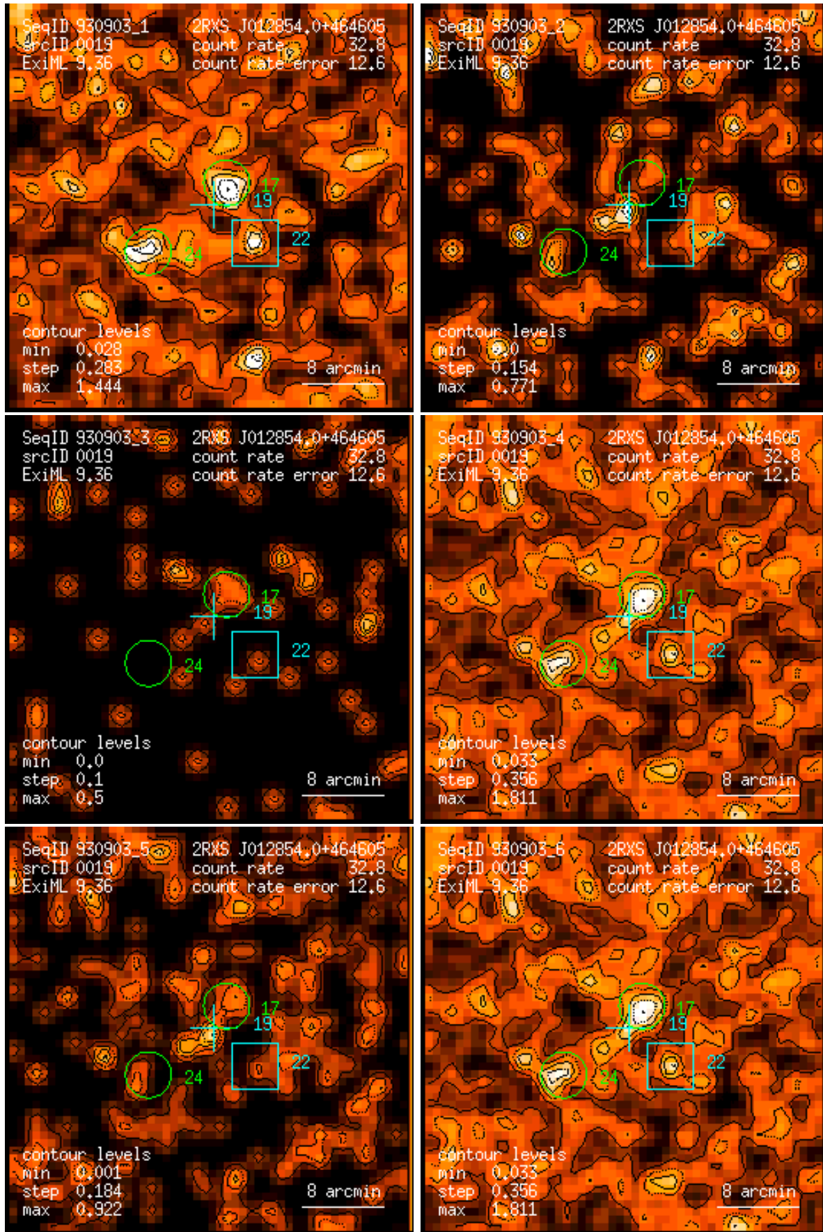
Figure 19: RASS 930903: detection 0019: band rate images, Gaussian filter: (1) PSPC channels 11 – 41, (2) 52 – 90, (3) 91 – 201, (4) 11 – 235, (5) 52 – 201, (6) 11 – 201. Broad band rates in counts/ks. Band rate contour levels in counts/ks/arcmin 2 .
