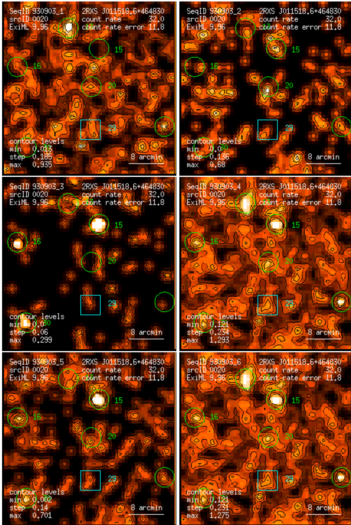
Figure 20: RASS 930903: detection 0020: band rate images, Gaussian filter: (1) PSPC channels 11 – 41, (2) 52 – 90, (3) 91 – 201, (4) 11 – 235, (5) 52 – 201, (6) 11 – 201. Broad band rates in counts/ks. Band rate contour levels in counts/ks/arcmin 2 .
