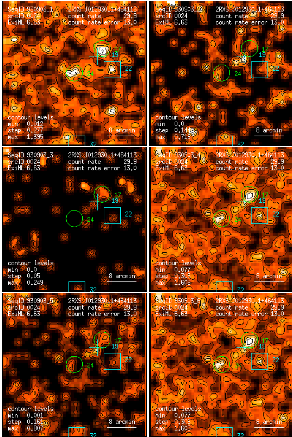
Figure 24: RASS 930903: detection 0024: band rate images, Gaussian filter: (1) PSPC channels 11 – 41, (2) 52 – 90, (3) 91 – 201, (4) 11 – 235, (5) 52 – 201, (6) 11 – 201. Broad band rates in counts/ks. Band rate contour levels in counts/ks/arcmin 2 .
