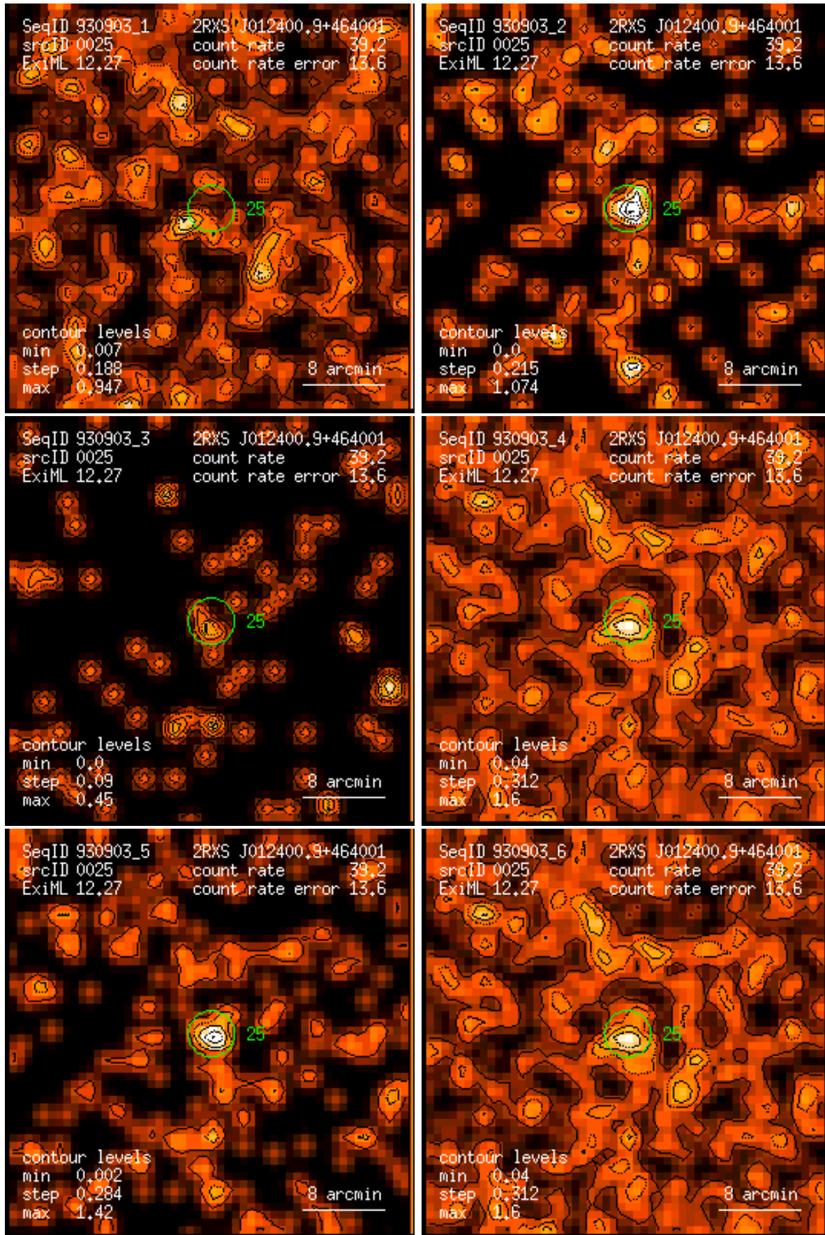
Figure 25: RASS 930903: detection 0025: band rate images, Gaussian filter: (1) PSPC channels 11 – 41, (2) 52 – 90, (3) 91 – 201, (4) 11 – 235, (5) 52 – 201, (6) 11 – 201. Broad band rates in counts/ks. Band rate contour levels in counts/ks/arcmin 2 .
