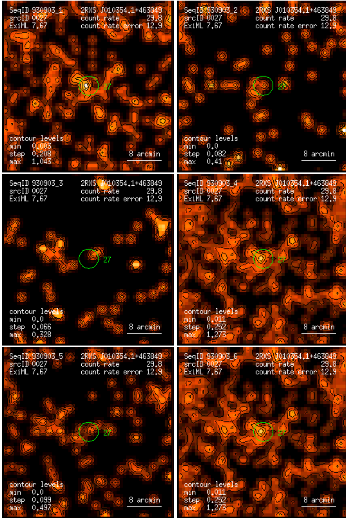
Figure 27: RASS 930903: detection 0027: band rate images, Gaussian filter: (1) PSPC channels 11 – 41, (2) 52 – 90, (3) 91 – 201, (4) 11 – 235, (5) 52 – 201, (6) 11 – 201. Broad band rates in counts/ks. Band rate contour levels in counts/ks/arcmin 2 .
