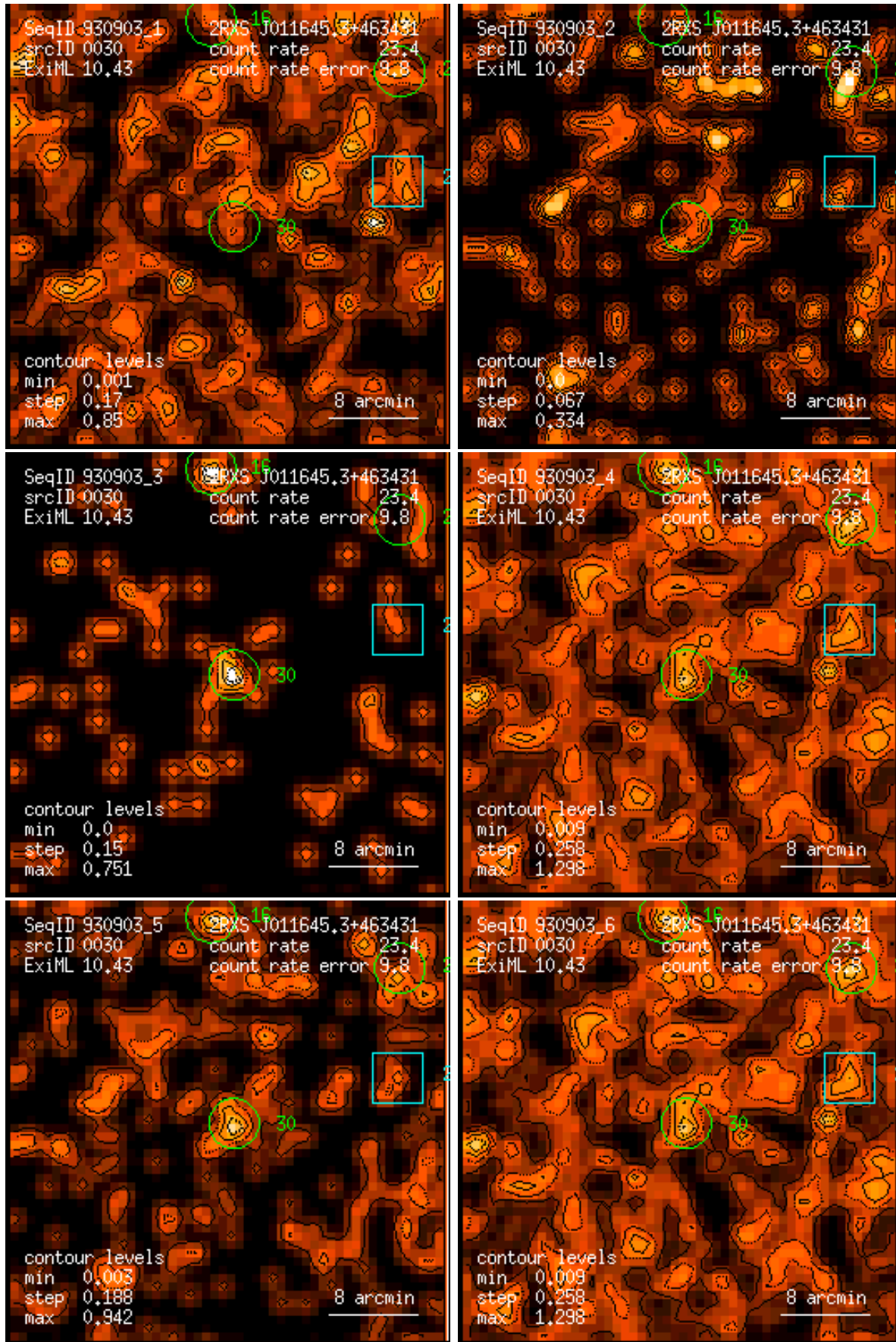
Figure 30: RASS 930903: detection 0030: band rate images, Gaussian filter: (1) PSPC channels 11 – 41, (2) 52 – 90, (3) 91 – 201, (4) 11 – 235, (5) 52 – 201, (6) 11 – 201. Broad band rates in counts/ks. Band rate contour levels in counts/ks/arcmin 2 .
