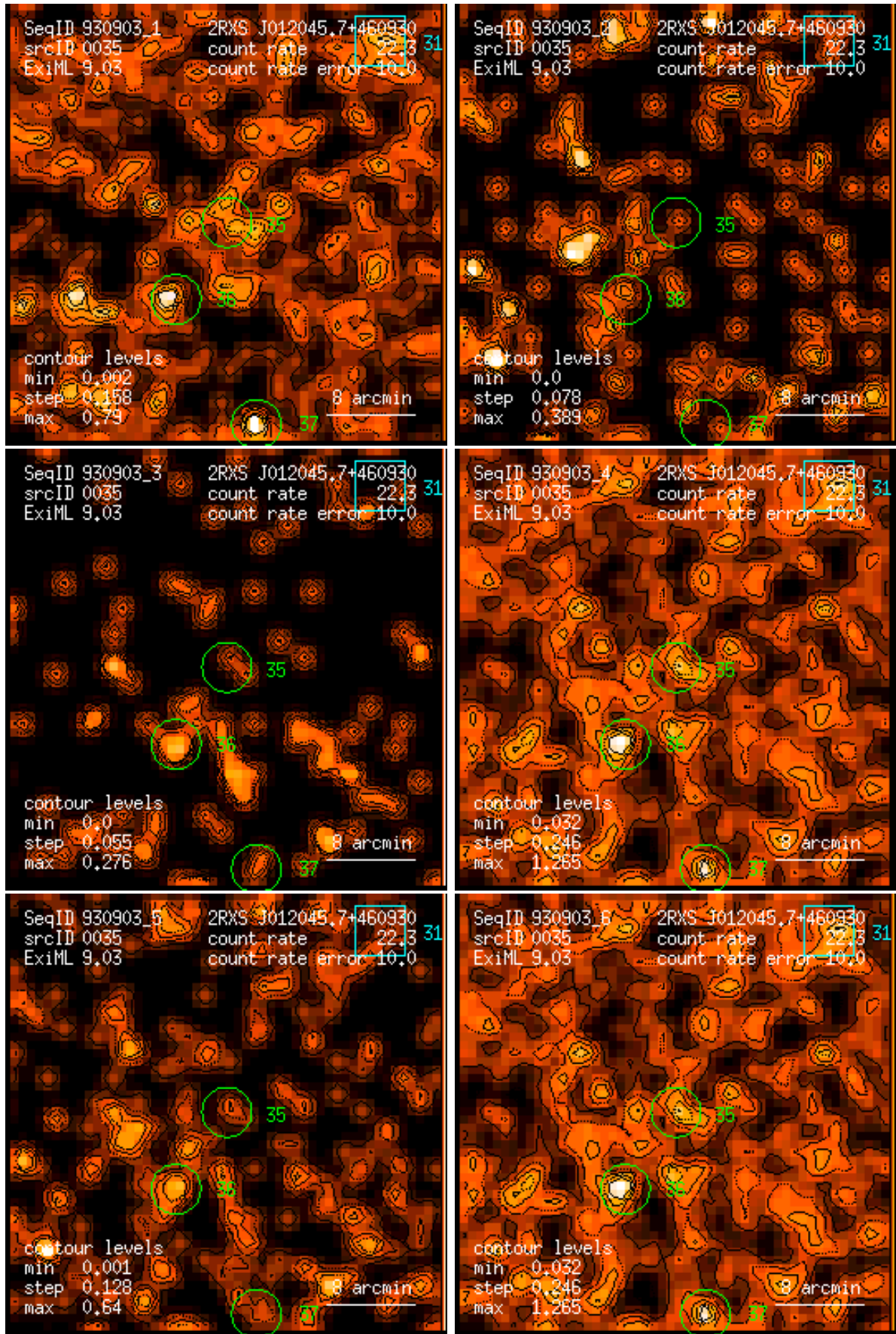
Figure 35: RASS 930903: detection 0035: band rate images, Gaussian filter: (1) PSPC channels 11 – 41, (2) 52 – 90, (3) 91 – 201, (4) 11 – 235, (5) 52 – 201, (6) 11 – 201. Broad band rates in counts/ks. Band rate contour levels in counts/ks/arcmin 2 .
