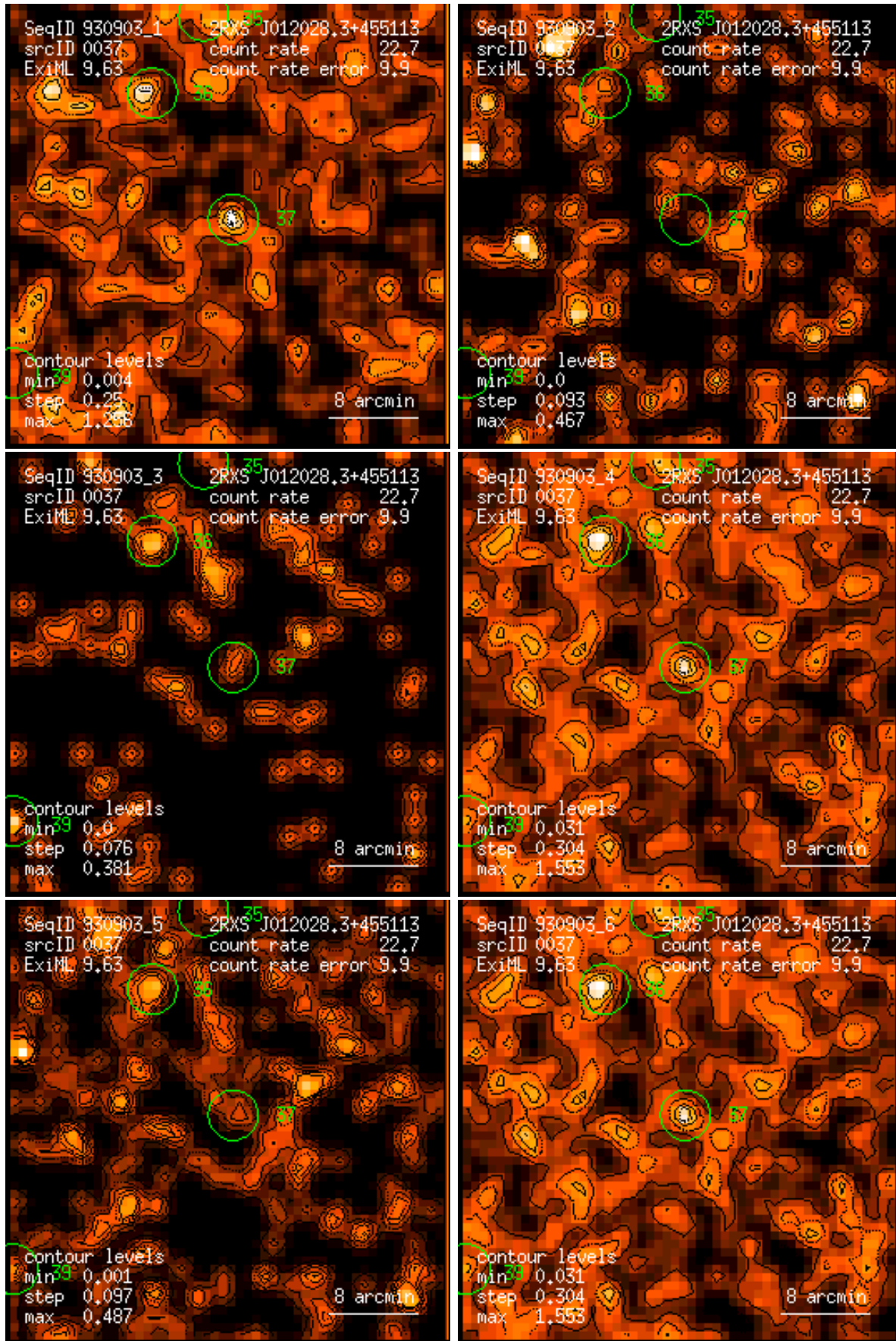
Figure 37: RASS 930903: detection 0037: band rate images, Gaussian filter: (1) PSPC channels 11 – 41, (2) 52 – 90, (3) 91 – 201, (4) 11 – 235, (5) 52 – 201, (6) 11 – 201. Broad band rates in counts/ks. Band rate contour levels in counts/ks/arcmin 2 .
