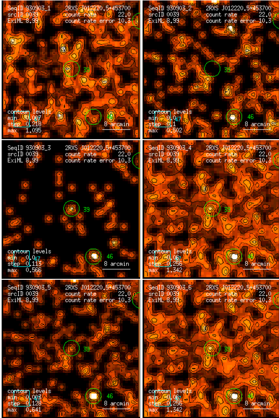
Figure 39: RASS 930903: detection 0039: band rate images, Gaussian filter: (1) PSPC channels 11 – 41, (2) 52 – 90, (3) 91 – 201, (4) 11 – 235, (5) 52 – 201, (6) 11 – 201. Broad band rates in counts/ks. Band rate contour levels in counts/ks/arcmin 2 .
