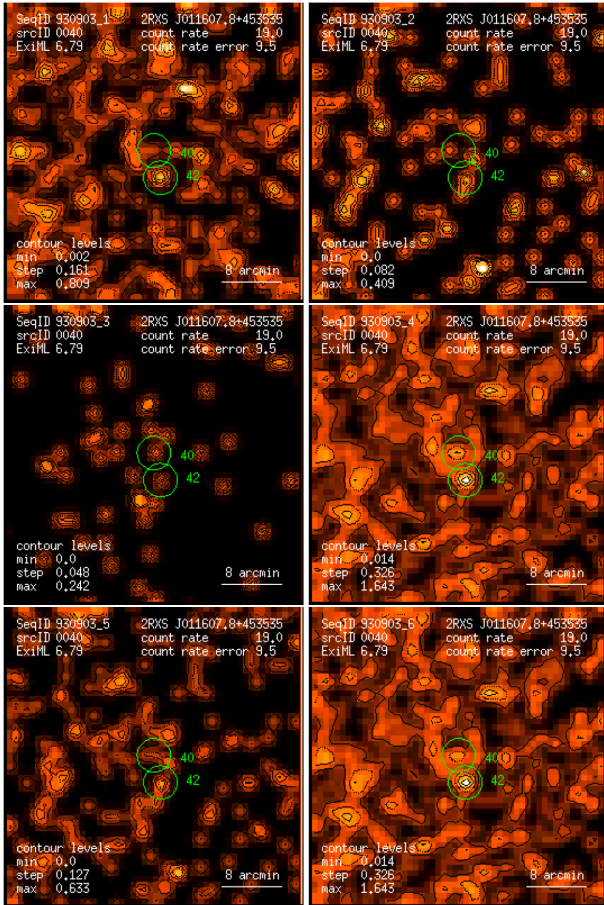
Figure 40: RASS 930903: detection 0040: band rate images, Gaussian filter: (1) PSPC channels 11 – 41, (2) 52 – 90, (3) 91 – 201, (4) 11 – 235, (5) 52 – 201, (6) 11 – 201. Broad band rates in counts/ks. Band rate contour levels in counts/ks/arcmin 2 .
