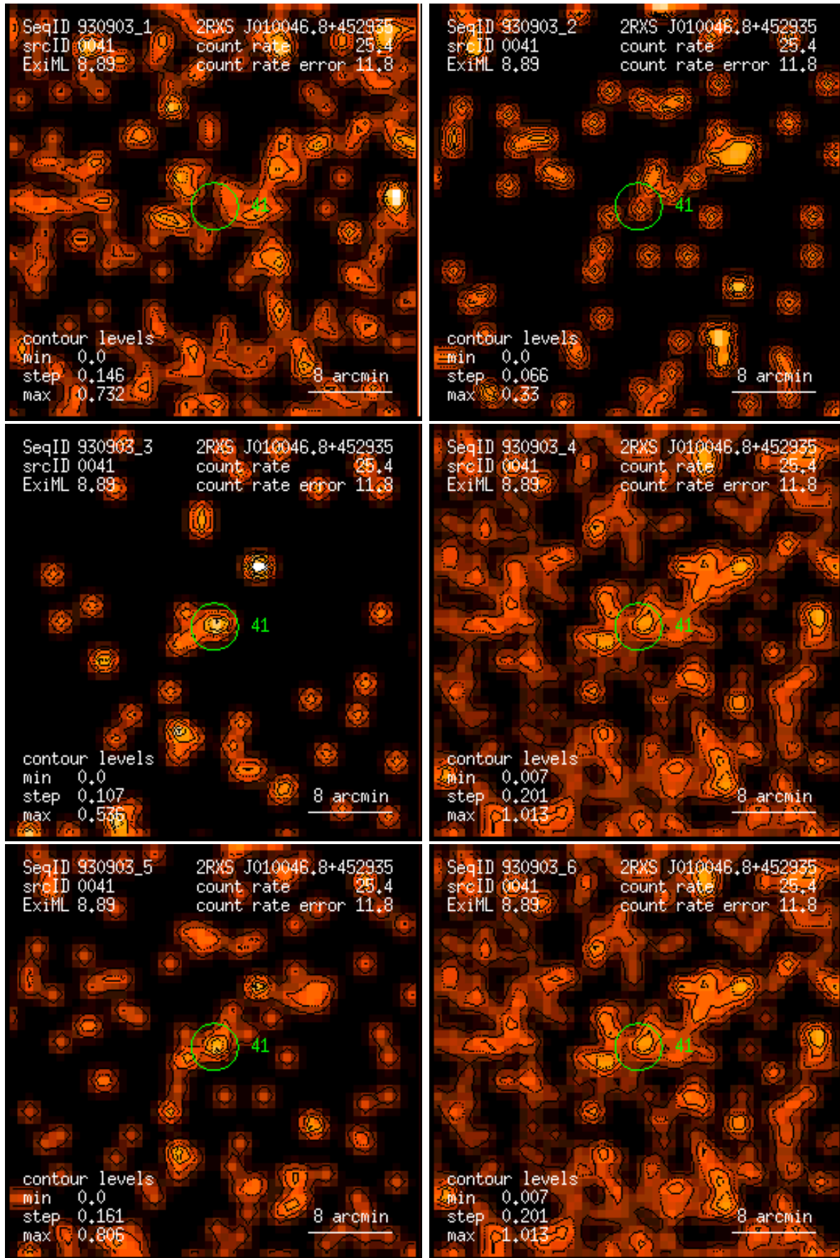
Figure 41: RASS 930903: detection 0041: band rate images, Gaussian filter: (1) PSPC channels 11 – 41, (2) 52 – 90, (3) 91 – 201, (4) 11 – 235, (5) 52 – 201, (6) 11 – 201. Broad band rates in counts/ks. Band rate contour levels in counts/ks/arcmin 2 .
