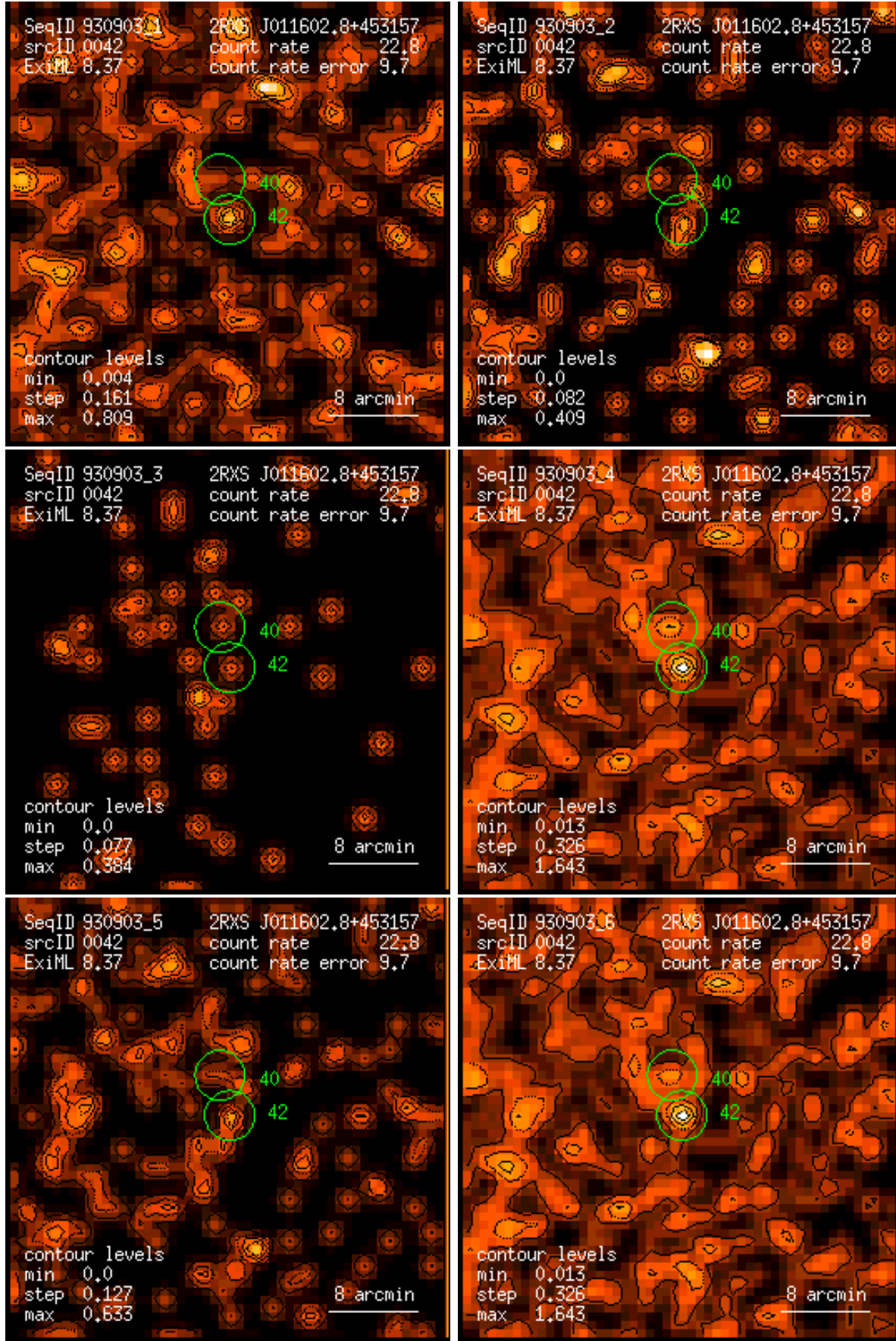
Figure 42: RASS 930903: detection 0042: band rate images, Gaussian filter: (1) PSPC channels 11 – 41, (2) 52 – 90, (3) 91 – 201, (4) 11 – 235, (5) 52 – 201, (6) 11 – 201. Broad band rates in counts/ks. Band rate contour levels in counts/ks/arcmin 2 .
