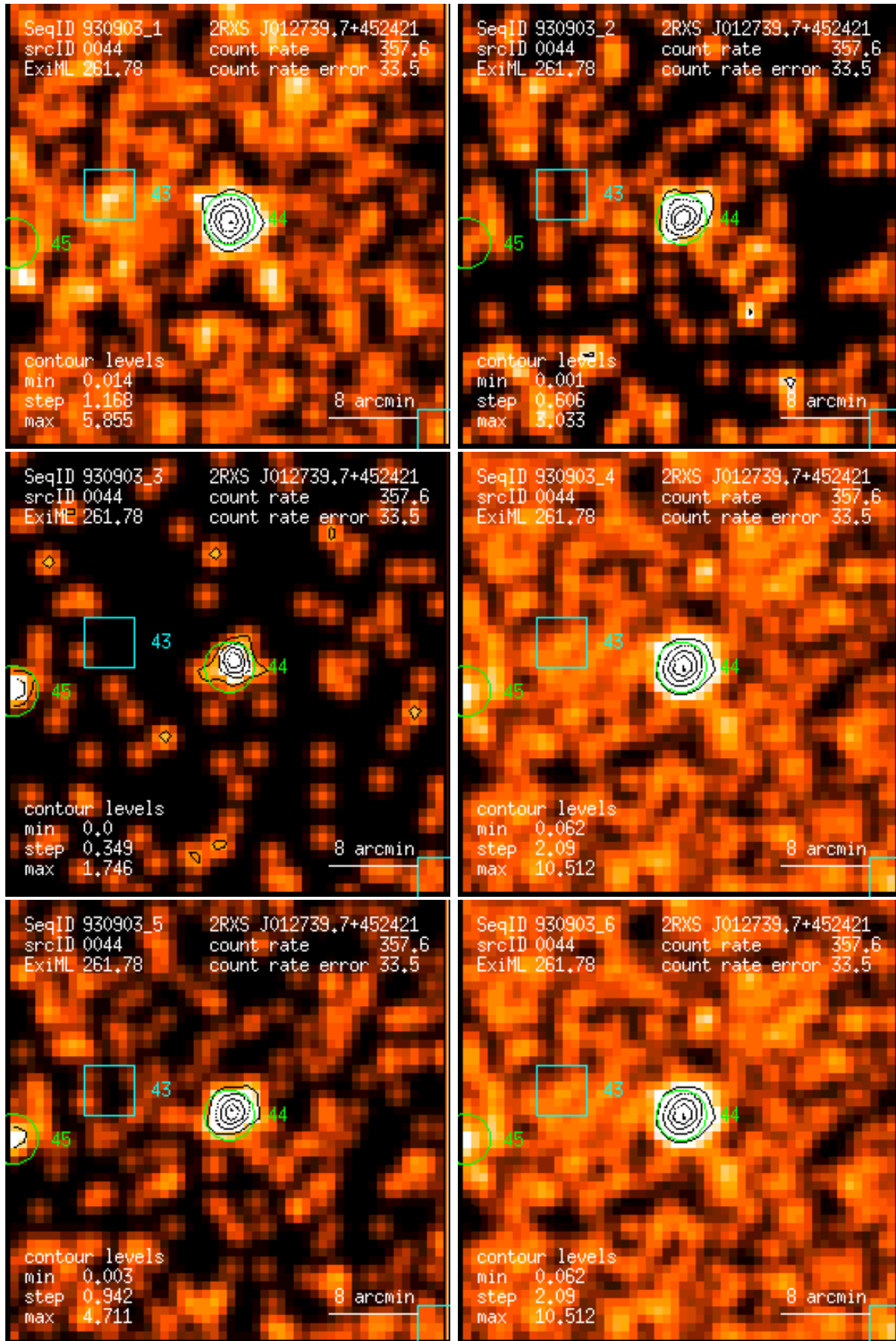
Figure 44: RASS 930903: detection 0044: band rate images, Gaussian filter: (1) PSPC channels 11 – 41, (2) 52 – 90, (3) 91 – 201, (4) 11 – 235, (5) 52 – 201, (6) 11 – 201. Broad band rates in counts/ks. Band rate contour levels in counts/ks/arcmin 2 .
