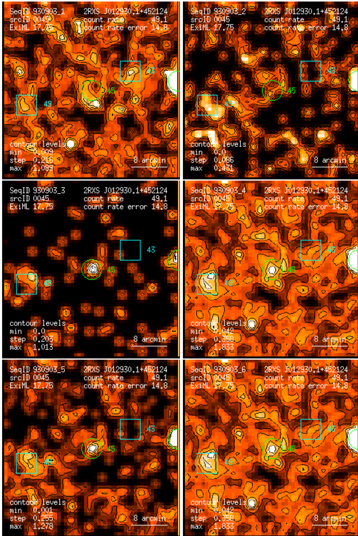
Figure 45: RASS 930903: detection 0045: band rate images, Gaussian filter: (1) PSPC channels 11 – 41, (2) 52 – 90, (3) 91 – 201, (4) 11 – 235, (5) 52 – 201, (6) 11 – 201. Broad band rates in counts/ks. Band rate contour levels in counts/ks/arcmin 2 .
