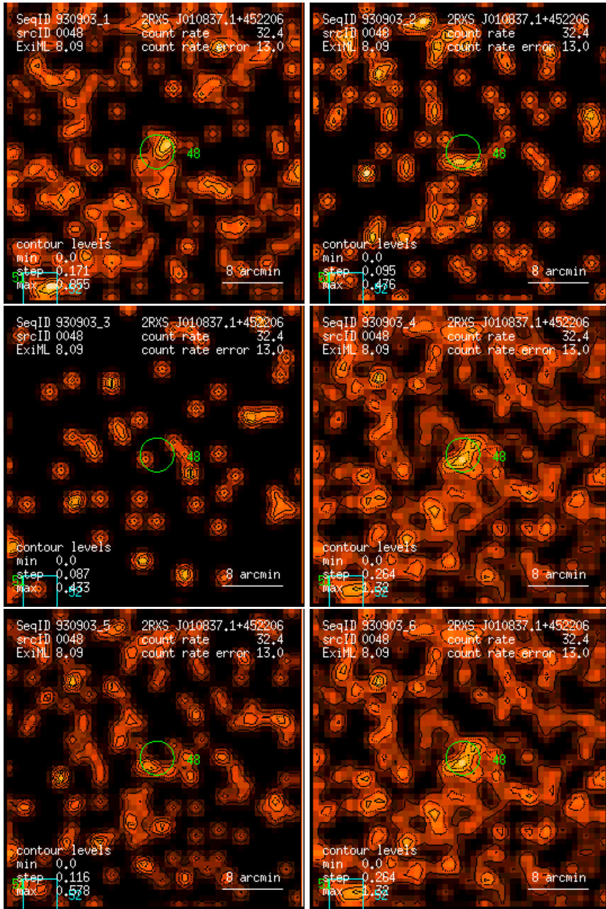
Figure 48: RASS 930903: detection 0048: band rate images, Gaussian filter: (1) PSPC channels 11 – 41, (2) 52 – 90, (3) 91 – 201, (4) 11 – 235, (5) 52 – 201, (6) 11 – 201. Broad band rates in counts/ks. Band rate contour levels in counts/ks/arcmin 2 .
