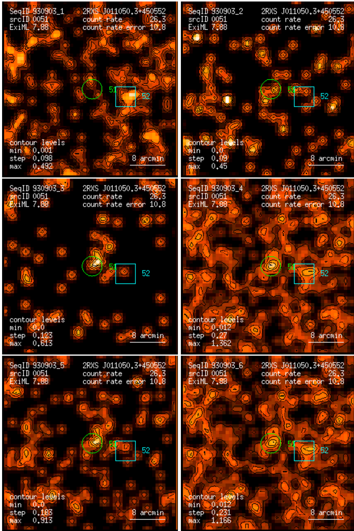
Figure 51: RASS 930903: detection 0051: band rate images, Gaussian filter: (1) PSPC channels 11 – 41, (2) 52 – 90, (3) 91 – 201, (4) 11 – 235, (5) 52 – 201, (6) 11 – 201. Broad band rates in counts/ks. Band rate contour levels in counts/ks/arcmin 2 .
