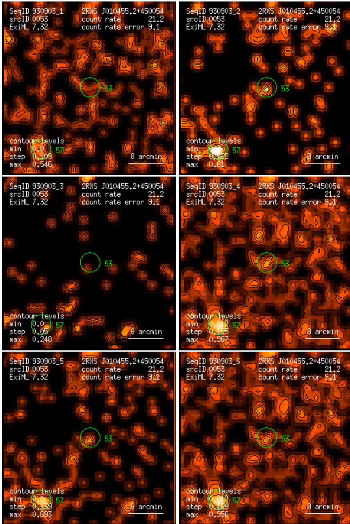
Figure 53: RASS 930903: detection 0053: band rate images, Gaussian filter: (1) PSPC channels 11 – 41, (2) 52 – 90, (3) 91 – 201, (4) 11 – 235, (5) 52 – 201, (6) 11 – 201. Broad band rates in counts/ks. Band rate contour levels in counts/ks/arcmin 2 .
