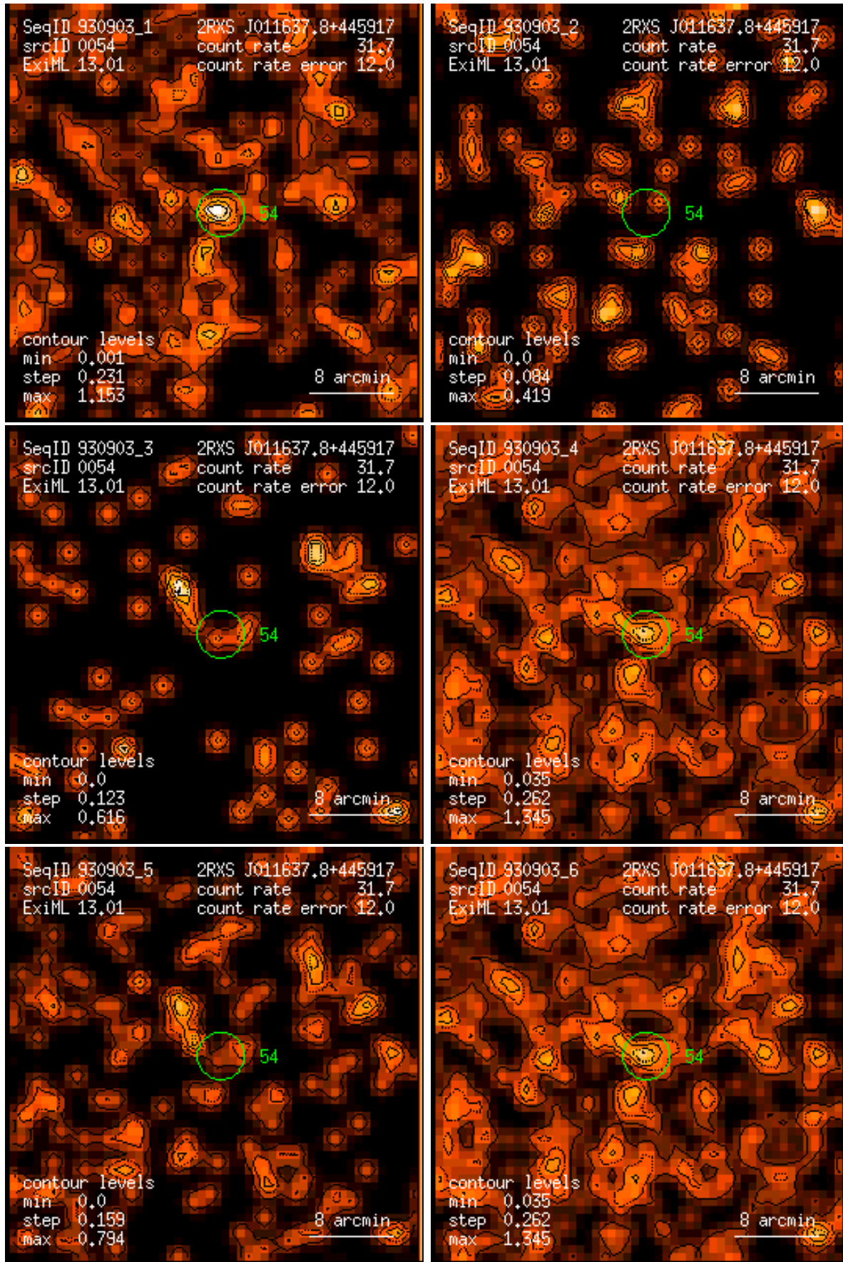
Figure 54: RASS 930903: detection 0054: band rate images, Gaussian filter: (1) PSPC channels 11 – 41, (2) 52 – 90, (3) 91 – 201, (4) 11 – 235, (5) 52 – 201, (6) 11 – 201. Broad band rates in counts/ks. Band rate contour levels in counts/ks/arcmin 2 .
