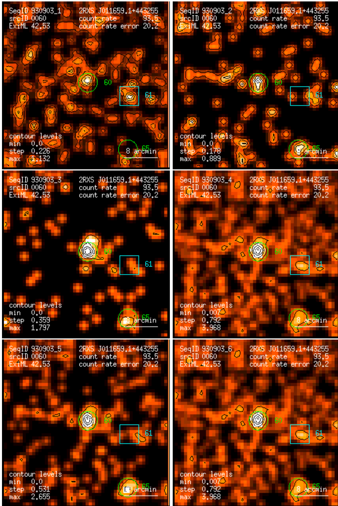
Figure 60: RASS 930903: detection 0060: band rate images, Gaussian filter: (1) PSPC channels 11 – 41, (2) 52 – 90, (3) 91 – 201, (4) 11 – 235, (5) 52 – 201, (6) 11 – 201. Broad band rates in counts/ks. Band rate contour levels in counts/ks/arcmin 2 .
