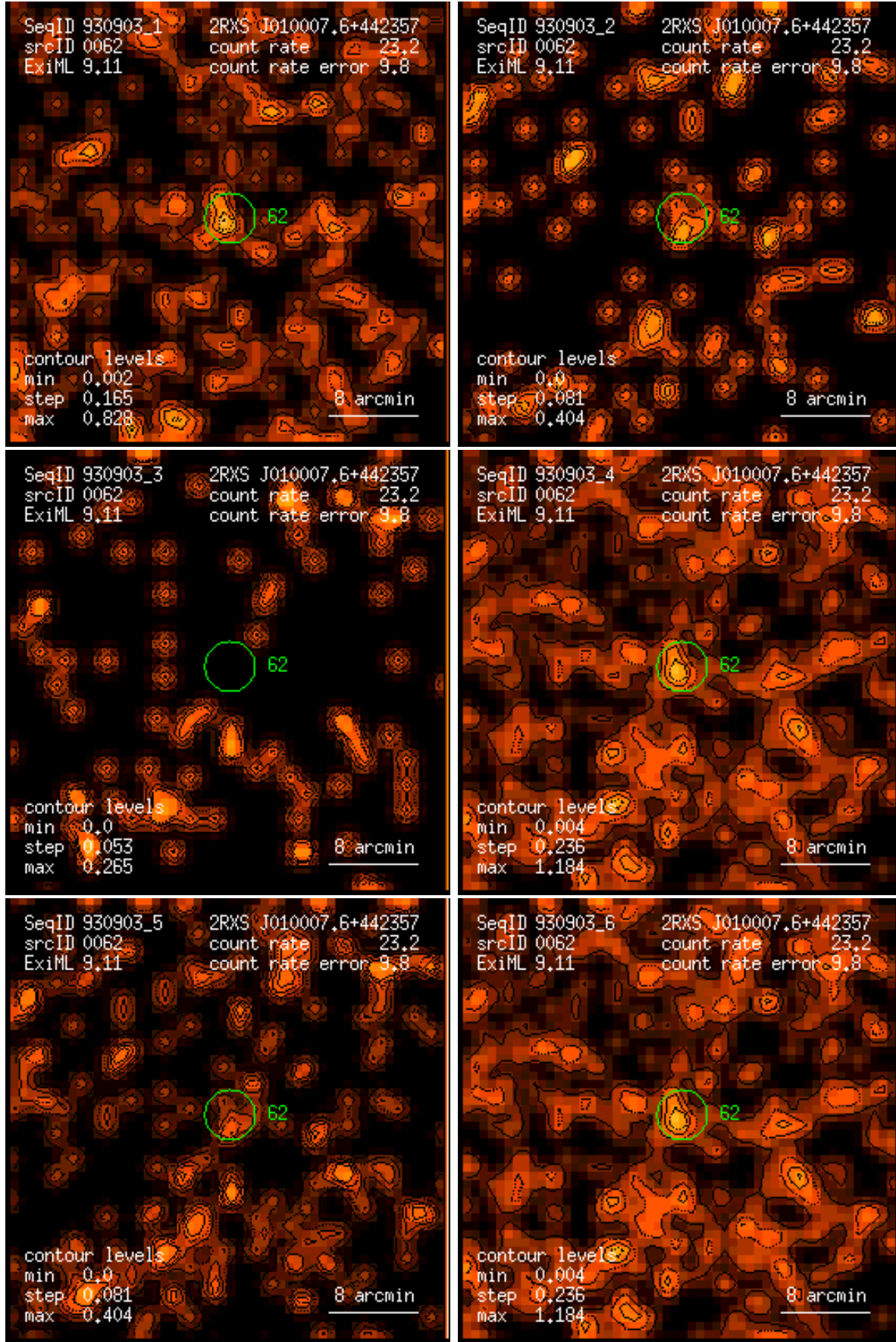
Figure 62: RASS 930903: detection 0062: band rate images, Gaussian filter: (1) PSPC channels 11 – 41, (2) 52 – 90, (3) 91 – 201, (4) 11 – 235, (5) 52 – 201, (6) 11 – 201. Broad band rates in counts/ks. Band rate contour levels in counts/ks/arcmin 2 .
