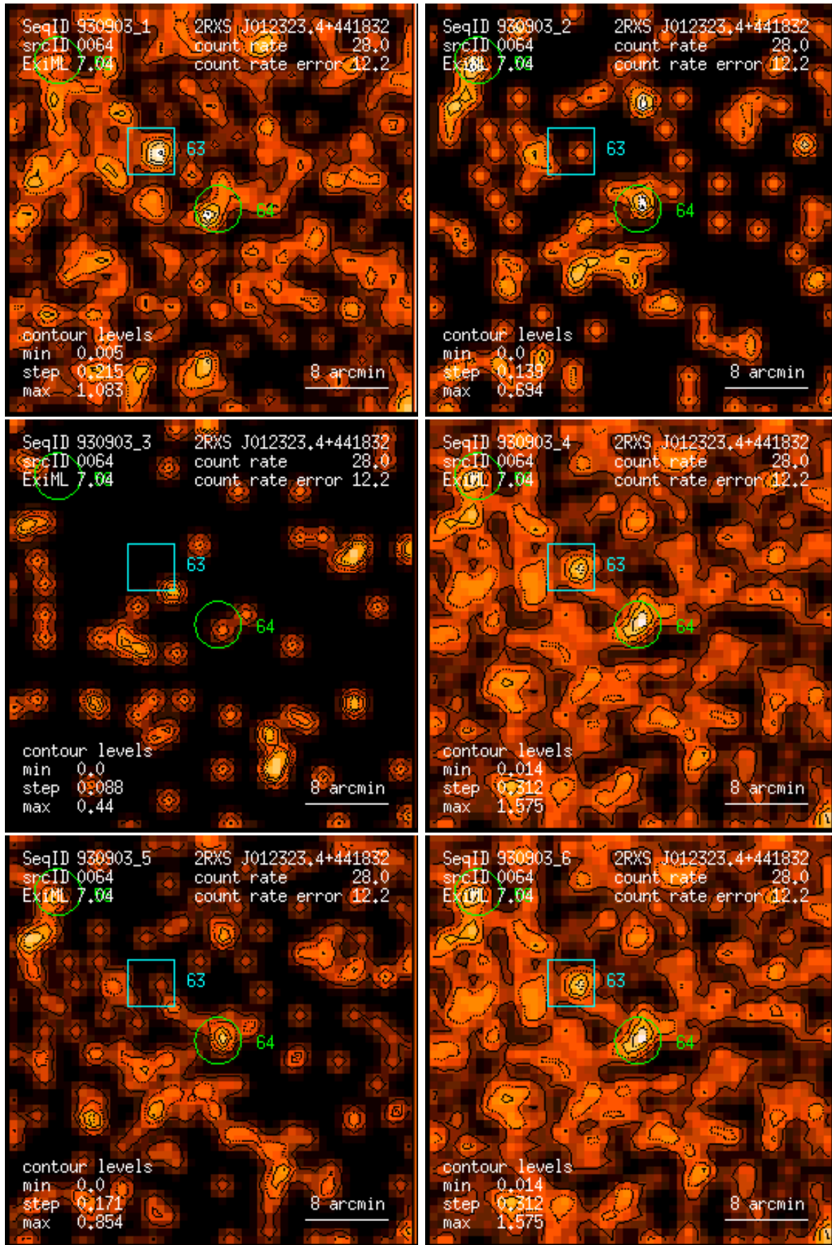
Figure 64: RASS 930903: detection 0064: band rate images, Gaussian filter: (1) PSPC channels 11 – 41, (2) 52 – 90, (3) 91 – 201, (4) 11 – 235, (5) 52 – 201, (6) 11 – 201. Broad band rates in counts/ks. Band rate contour levels in counts/ks/arcmin 2 .
