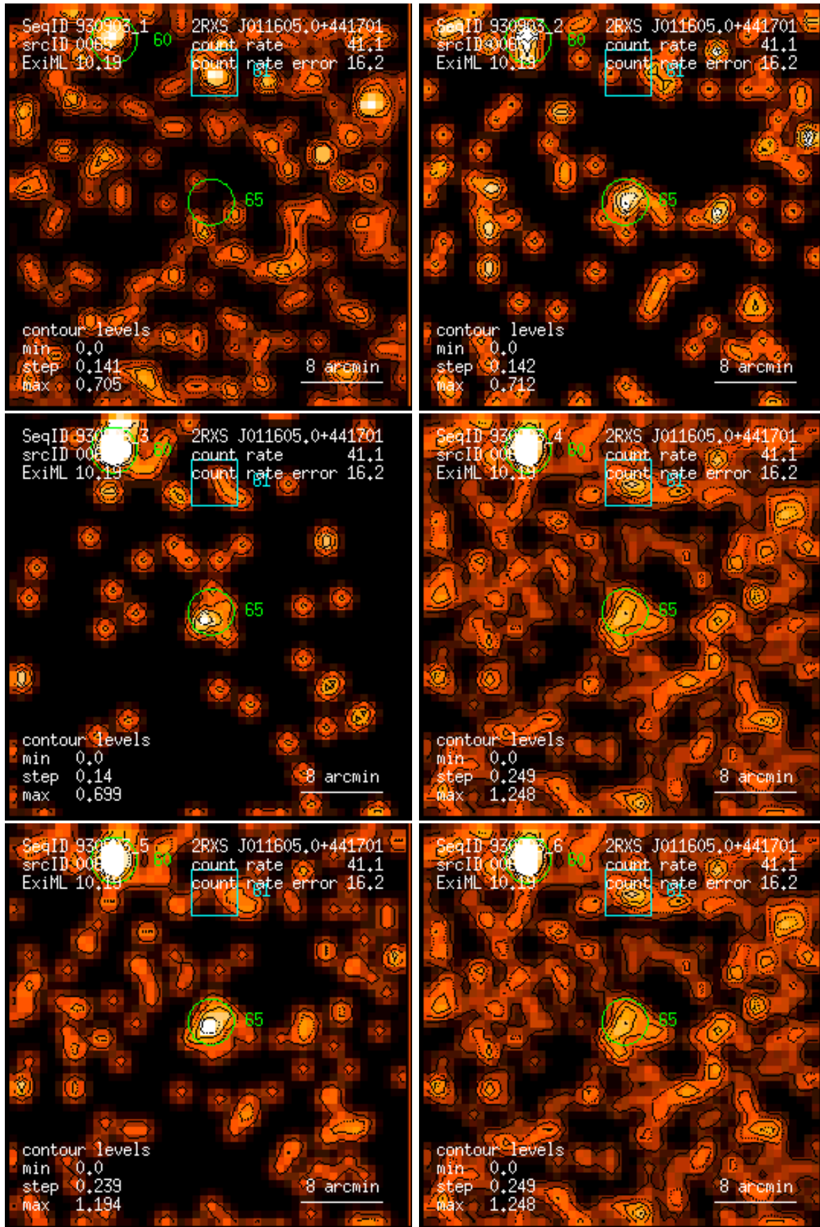
Figure 65: RASS 930903: detection 0065: band rate images, Gaussian filter: (1) PSPC channels 11 – 41, (2) 52 – 90, (3) 91 – 201, (4) 11 – 235, (5) 52 – 201, (6) 11 – 201. Broad band rates in counts/ks. Band rate contour levels in counts/ks/arcmin 2 .
