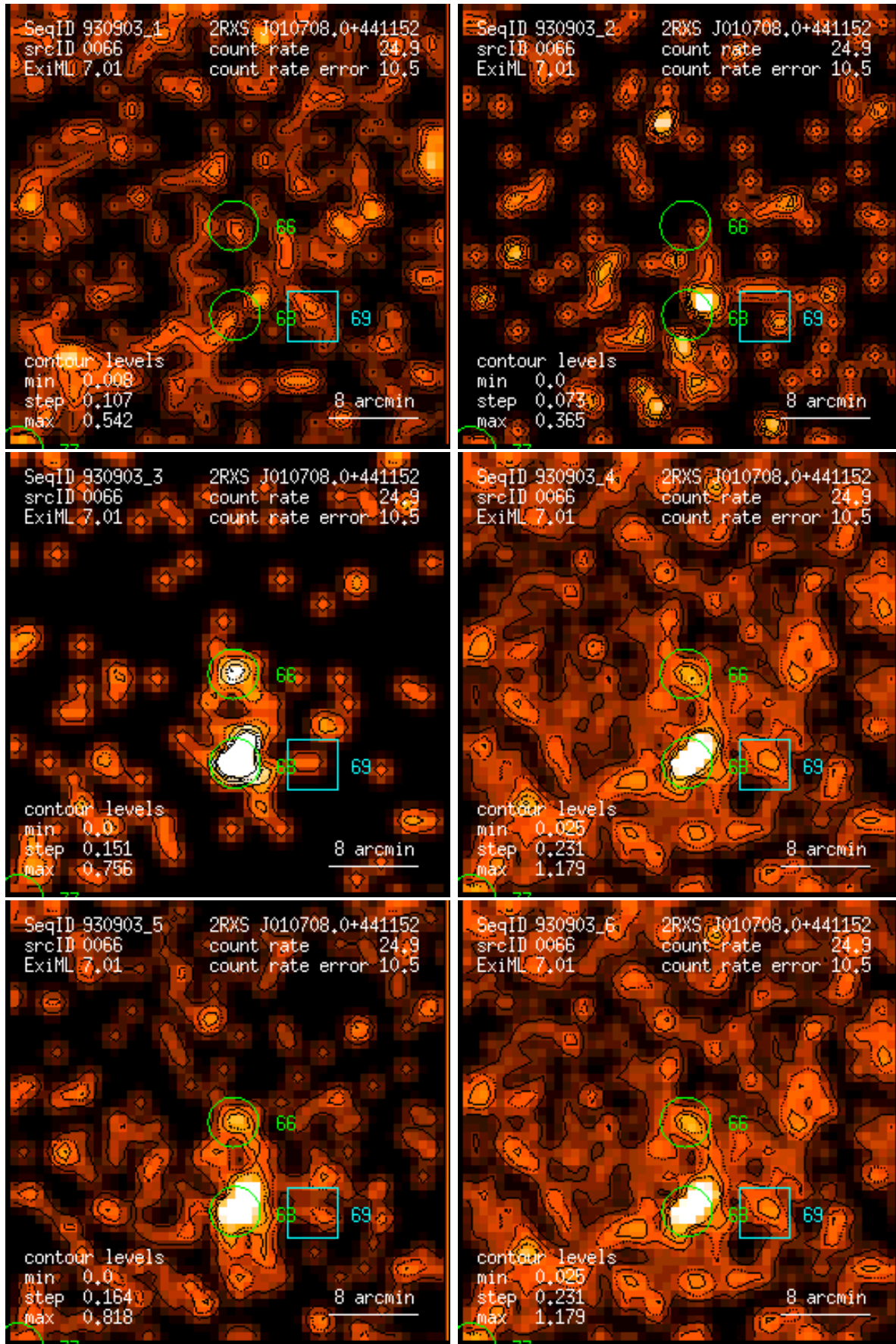
Figure 66: RASS 930903: detection 0066: band rate images, Gaussian filter: (1) PSPC channels 11 – 41, (2) 52 – 90, (3) 91 – 201, (4) 11 – 235, (5) 52 – 201, (6) 11 – 201. Broad band rates in counts/ks. Band rate contour levels in counts/ks/arcmin 2 .
