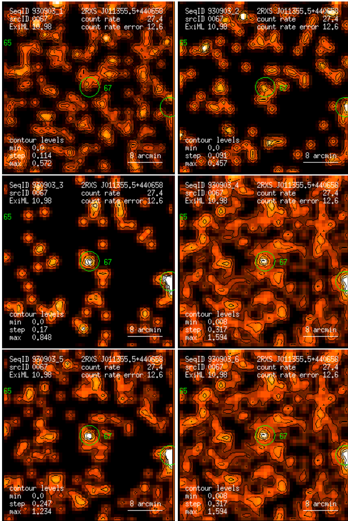
Figure 67: RASS 930903: detection 0067: band rate images, Gaussian filter: (1) PSPC channels 11 – 41, (2) 52 – 90, (3) 91 – 201, (4) 11 – 235, (5) 52 – 201, (6) 11 – 201. Broad band rates in counts/ks. Band rate contour levels in counts/ks/arcmin 2 .
