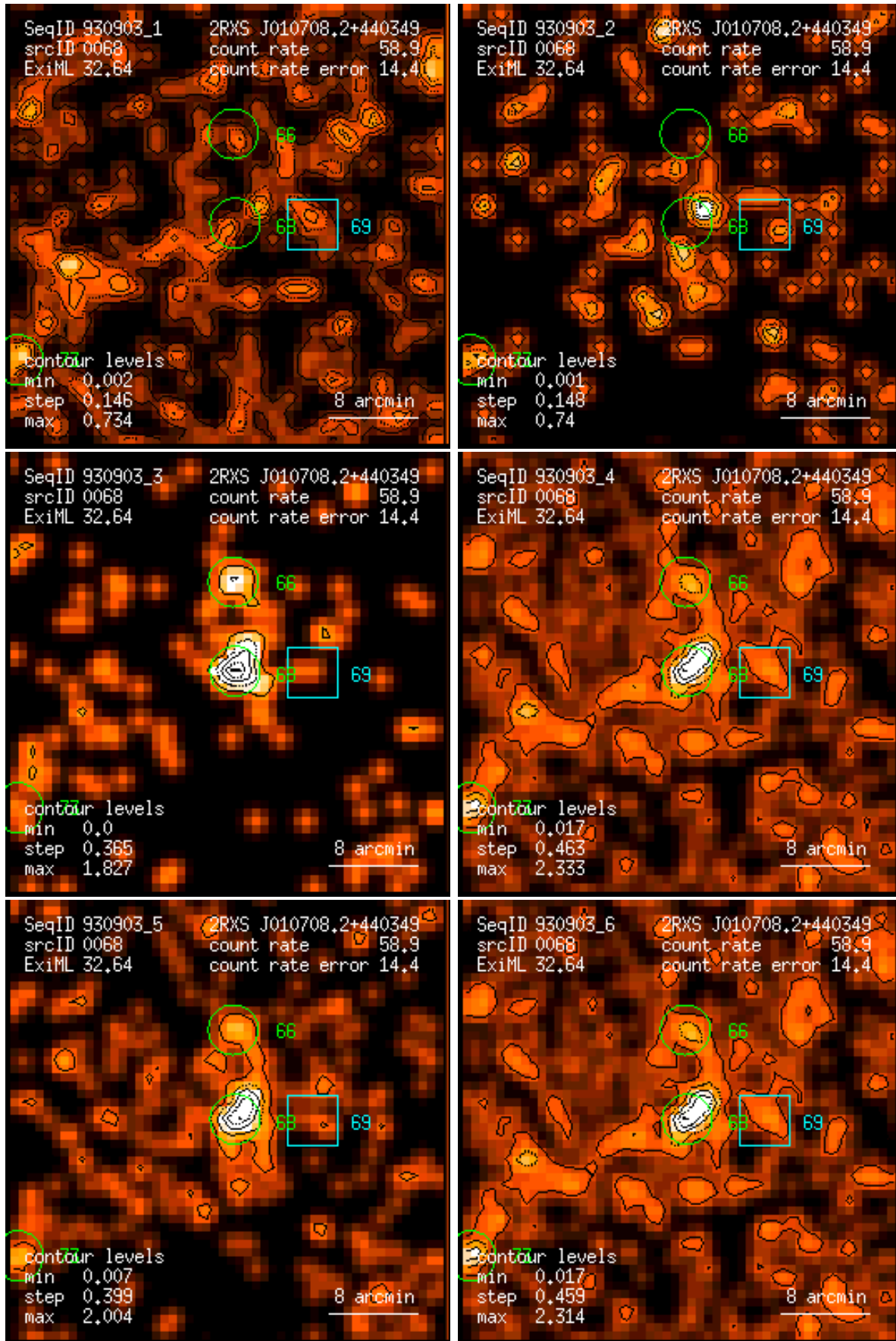
Figure 68: RASS 930903: detection 0068: band rate images, Gaussian filter: (1) PSPC channels 11 – 41, (2) 52 – 90, (3) 91 – 201, (4) 11 – 235, (5) 52 – 201, (6) 11 – 201. Broad band rates in counts/ks. Band rate contour levels in counts/ks/arcmin 2 .
