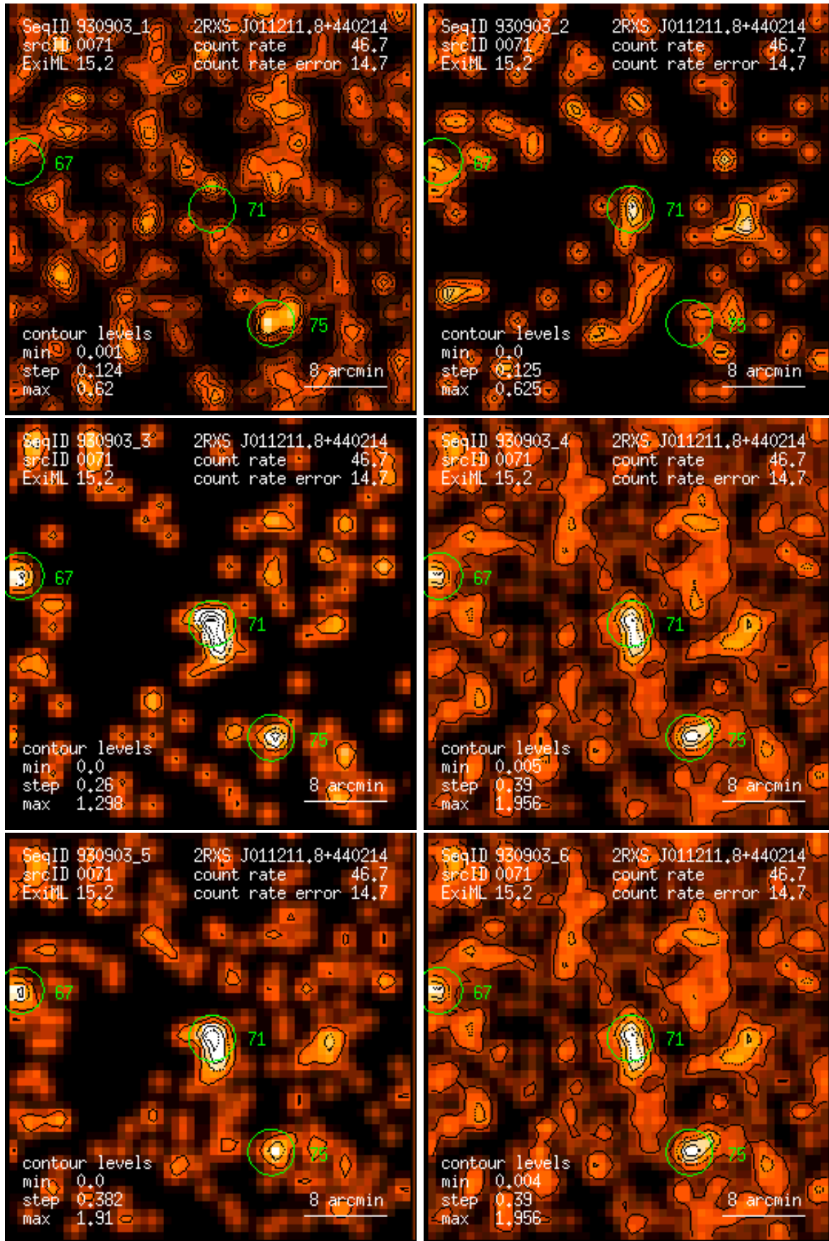
Figure 71: RASS 930903: detection 0071: band rate images, Gaussian filter: (1) PSPC channels 11 – 41, (2) 52 – 90, (3) 91 – 201, (4) 11 – 235, (5) 52 – 201, (6) 11 – 201. Broad band rates in counts/ks. Band rate contour levels in counts/ks/arcmin 2 .
