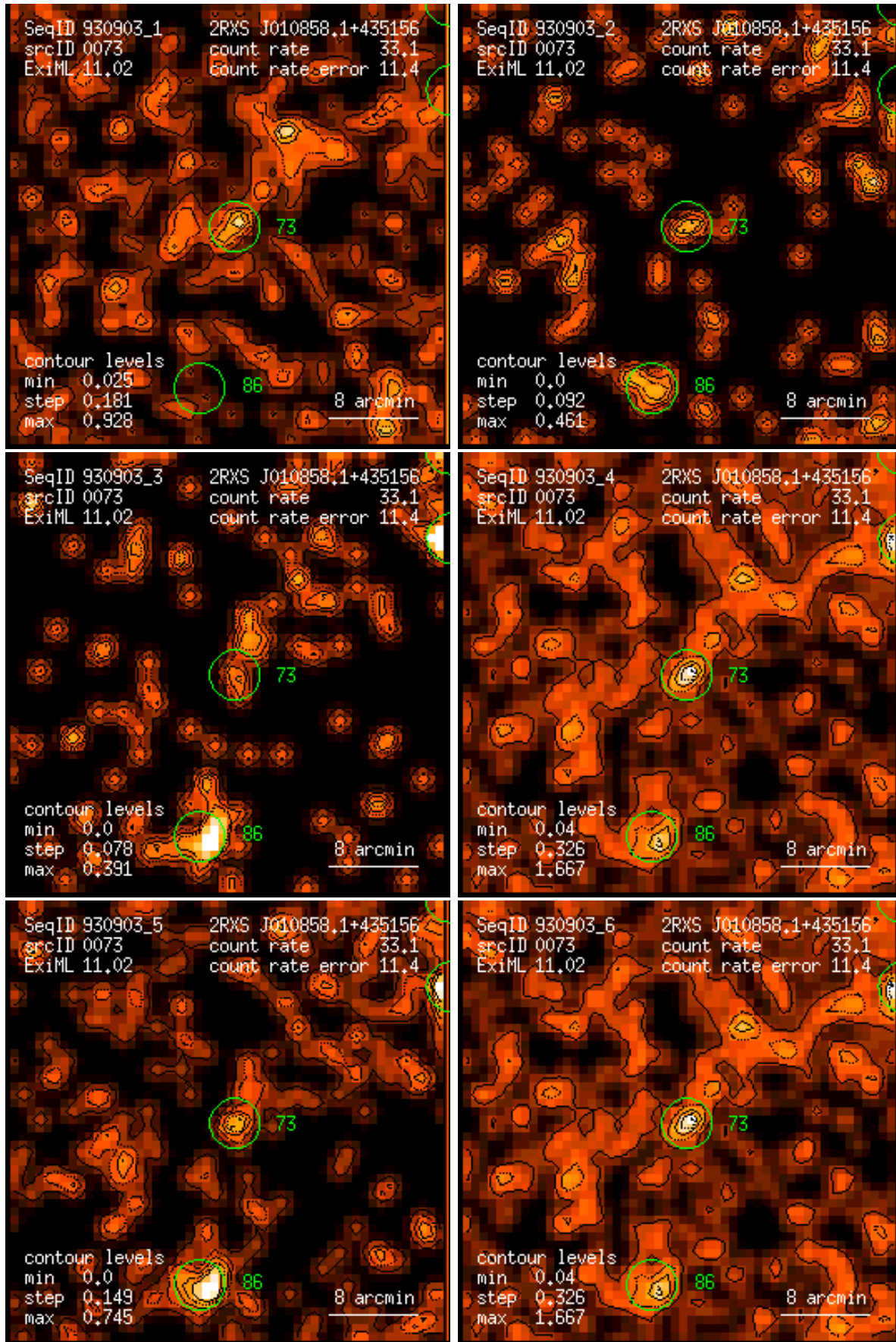
Figure 73: RASS 930903: detection 0073: band rate images, Gaussian filter: (1) PSPC channels 11 – 41, (2) 52 – 90, (3) 91 – 201, (4) 11 – 235, (5) 52 – 201, (6) 11 – 201. Broad band rates in counts/ks. Band rate contour levels in counts/ks/arcmin 2 .
