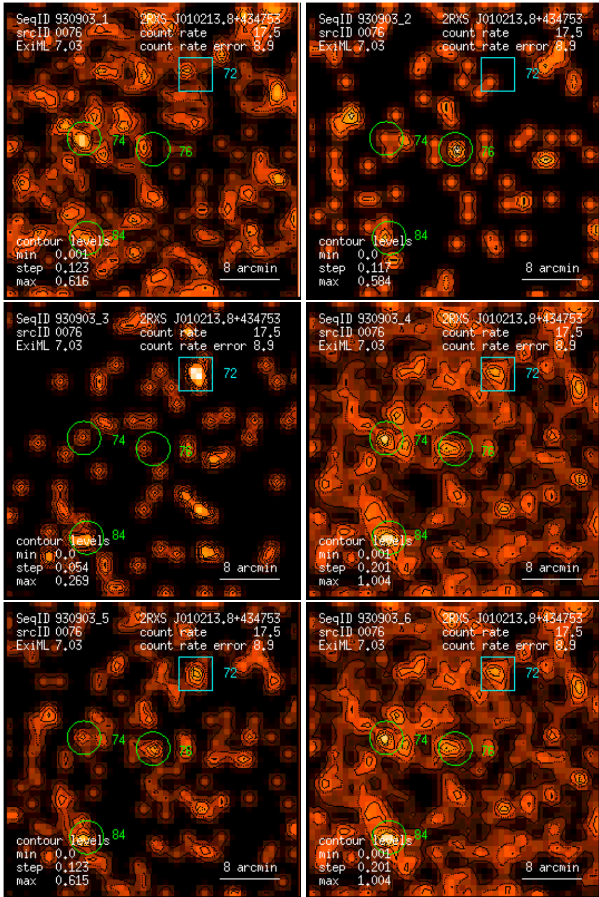
Figure 76: RASS 930903: detection 0076: band rate images, Gaussian filter: (1) PSPC channels 11 – 41, (2) 52 – 90, (3) 91 – 201, (4) 11 – 235, (5) 52 – 201, (6) 11 – 201. Broad band rates in counts/ks. Band rate contour levels in counts/ks/arcmin 2 .
