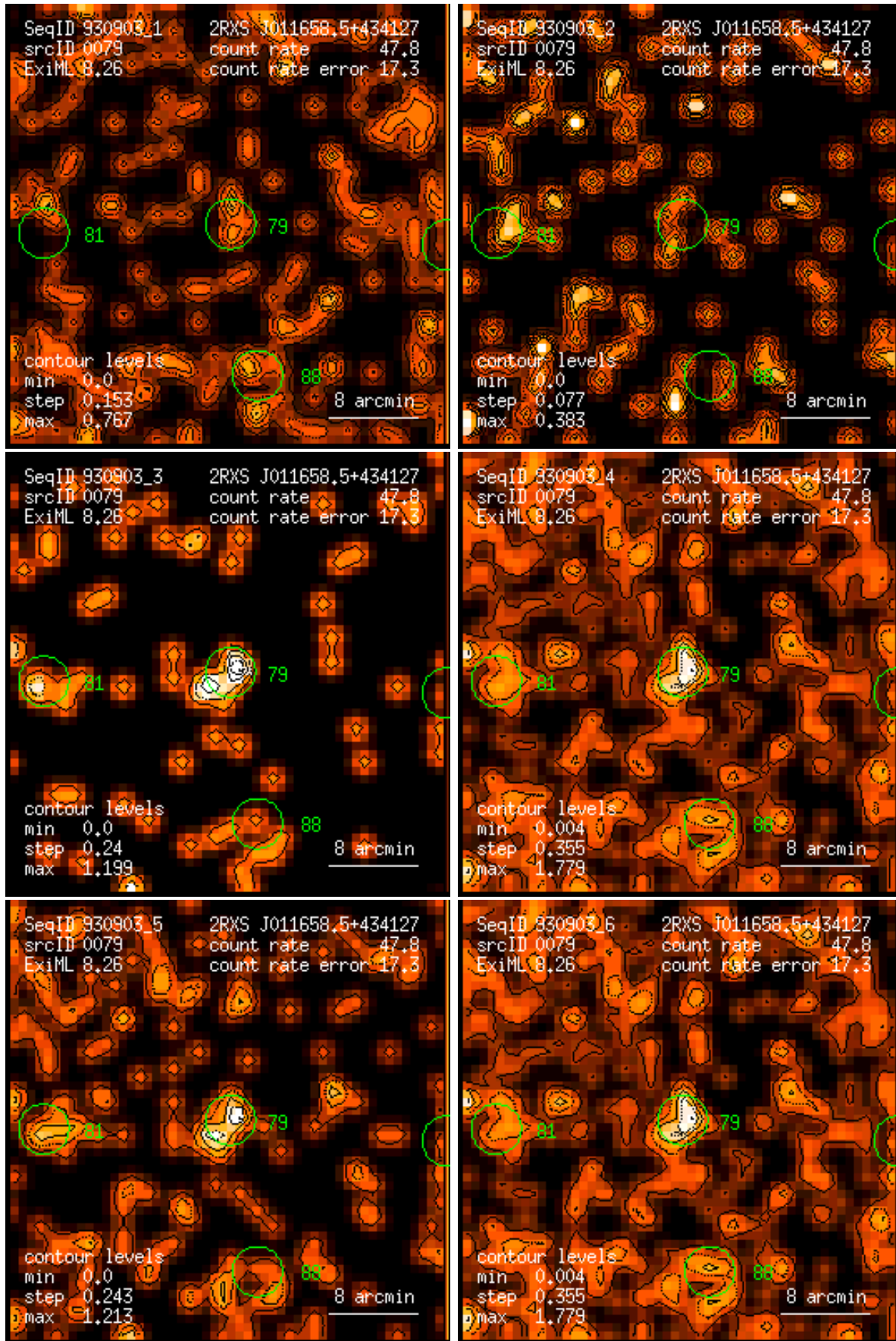
Figure 79: RASS 930903: detection 0079: band rate images, Gaussian filter: (1) PSPC channels 11 – 41, (2) 52 – 90, (3) 91 – 201, (4) 11 – 235, (5) 52 – 201, (6) 11 – 201. Broad band rates in counts/ks. Band rate contour levels in counts/ks/arcmin 2 .
