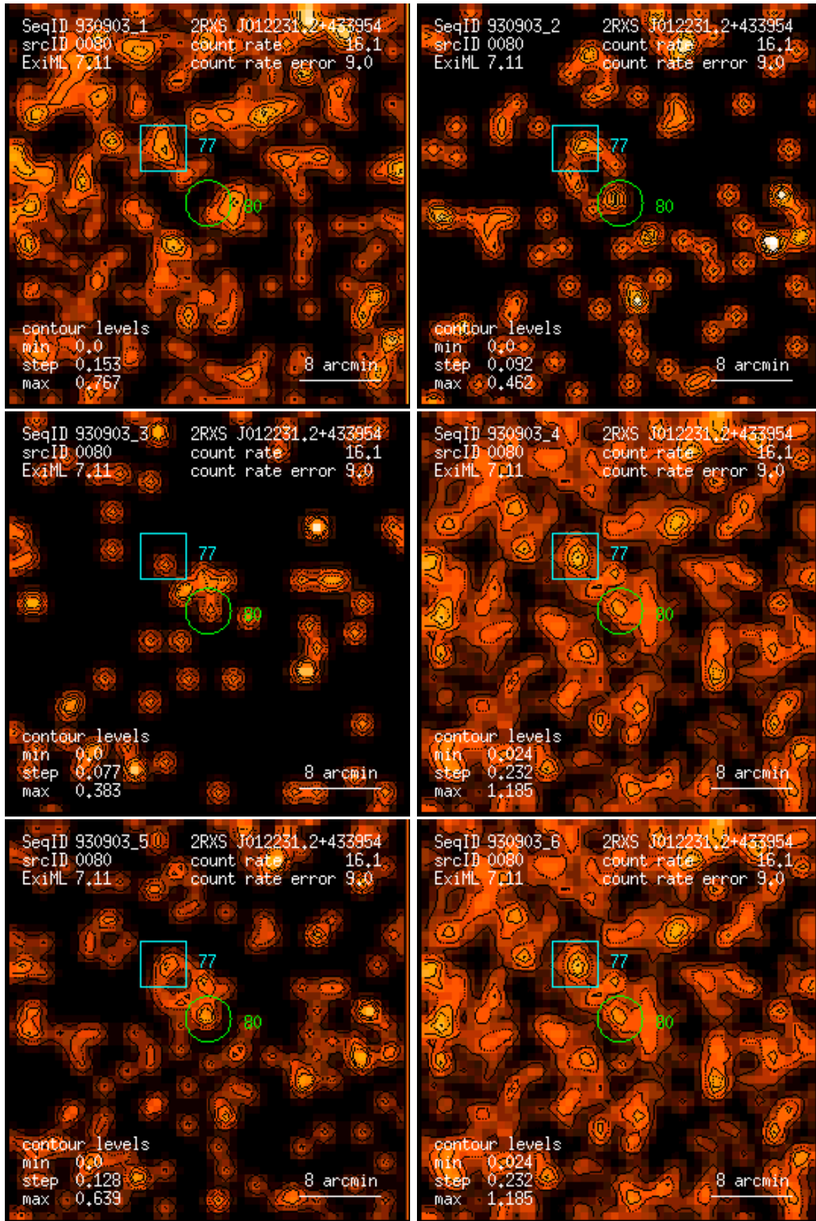
Figure 80: RASS 930903: detection 0080: band rate images, Gaussian filter: (1) PSPC channels 11 – 41, (2) 52 – 90, (3) 91 – 201, (4) 11 – 235, (5) 52 – 201, (6) 11 – 201. Broad band rates in counts/ks. Band rate contour levels in counts/ks/arcmin 2 .
