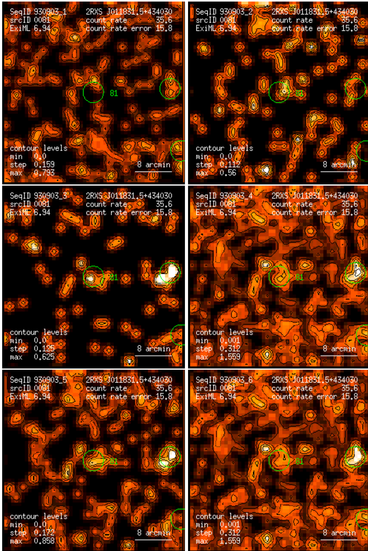
Figure 81: RASS 930903: detection 0081: band rate images, Gaussian filter: (1) PSPC channels 11 – 41, (2) 52 – 90, (3) 91 – 201, (4) 11 – 235, (5) 52 – 201, (6) 11 – 201. Broad band rates in counts/ks. Band rate contour levels in counts/ks/arcmin 2 .
