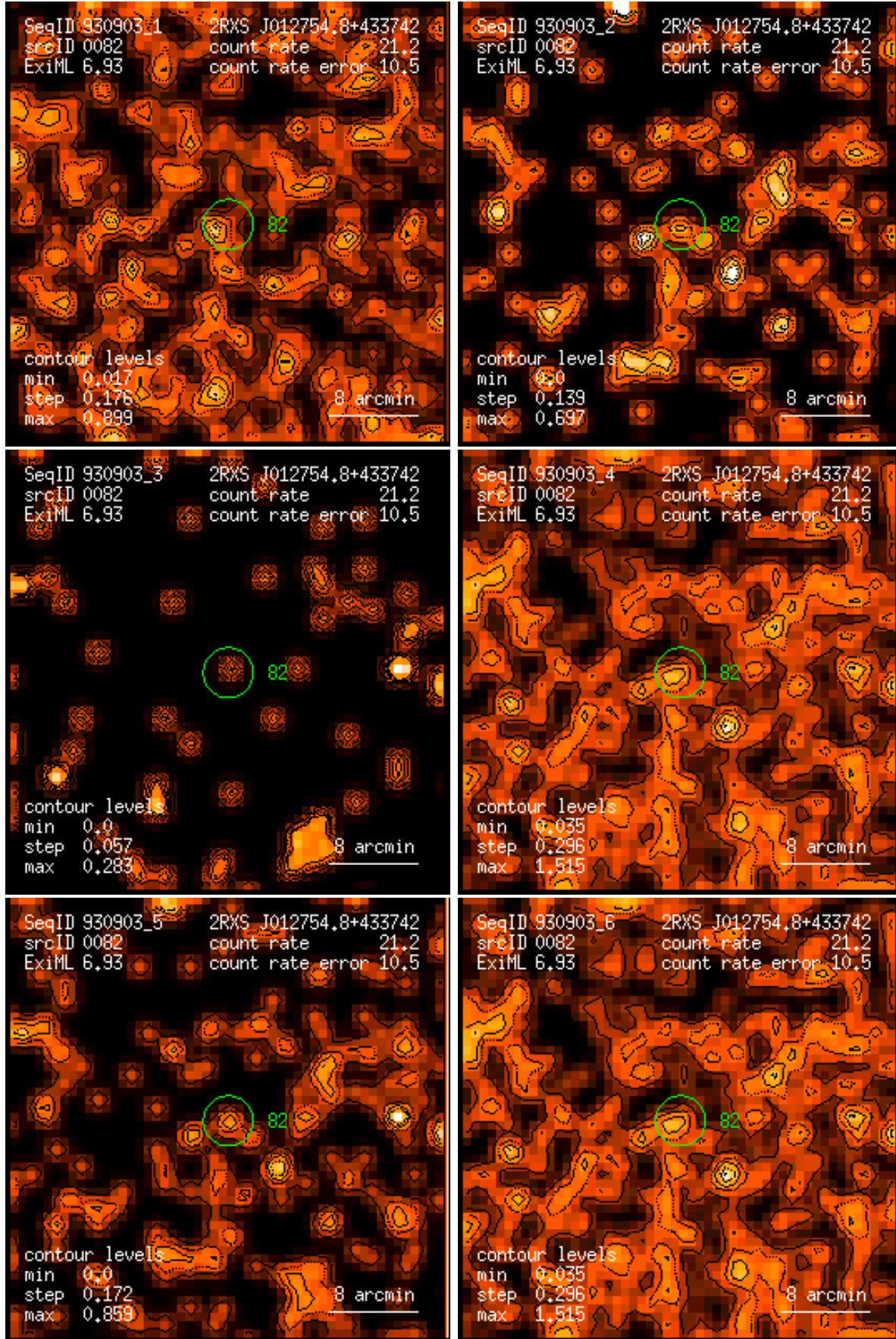
Figure 82: RASS 930903: detection 0082: band rate images, Gaussian filter: (1) PSPC channels 11 – 41, (2) 52 – 90, (3) 91 – 201, (4) 11 – 235, (5) 52 – 201, (6) 11 – 201. Broad band rates in counts/ks. Band rate contour levels in counts/ks/arcmin 2 .
