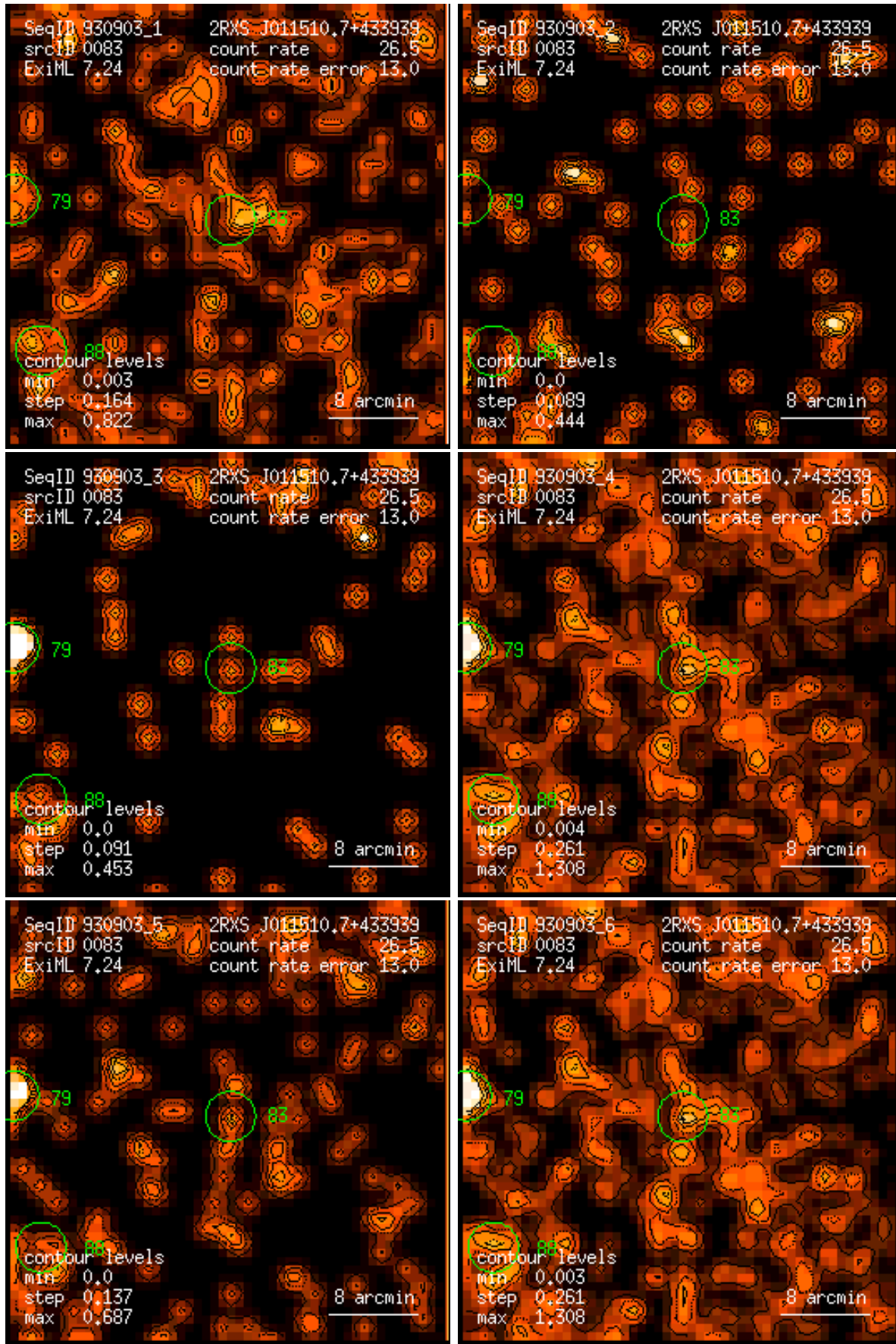
Figure 83: RASS 930903: detection 0083: band rate images, Gaussian filter: (1) PSPC channels 11 – 41, (2) 52 – 90, (3) 91 – 201, (4) 11 – 235, (5) 52 – 201, (6) 11 – 201. Broad band rates in counts/ks. Band rate contour levels in counts/ks/arcmin 2 .
