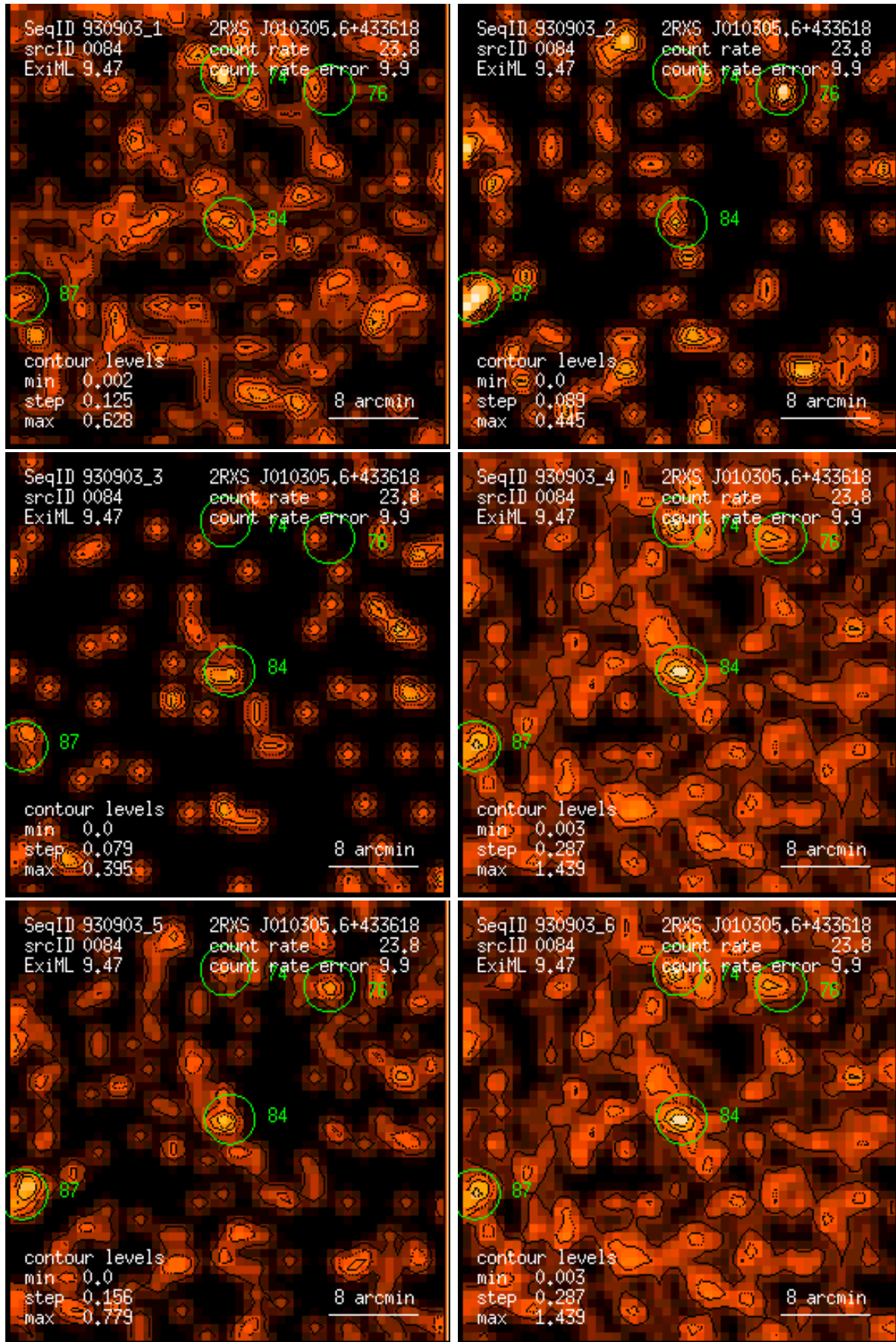
Figure 84: RASS 930903: detection 0084: band rate images, Gaussian filter: (1) PSPC channels 11 – 41, (2) 52 – 90, (3) 91 – 201, (4) 11 – 235, (5) 52 – 201, (6) 11 – 201. Broad band rates in counts/ks. Band rate contour levels in counts/ks/arcmin 2 .
