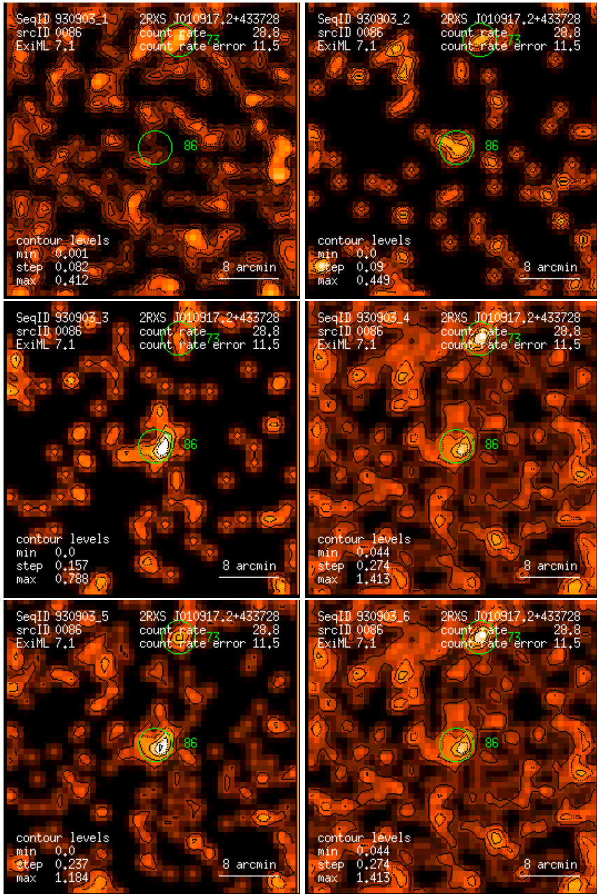
Figure 86: RASS 930903: detection 0086: band rate images, Gaussian filter: (1) PSPC channels 11 – 41, (2) 52 – 90, (3) 91 – 201, (4) 11 – 235, (5) 52 – 201, (6) 11 – 201. Broad band rates in counts/ks. Band rate contour levels in counts/ks/arcmin 2 .
